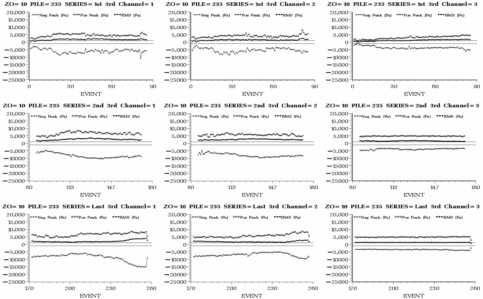
Figure C.10. Peak Positive, Peak Negative, and Root Mean Square Sound Pressure (Pa) of Each Impact on Plumb Pile 235 Driven at Hood Canal Bridge in 4.5 ft of Water with a Type II Confined Bubble Curtain in Place. Plots are arranged by hydrophone H1 (left) to H3 (right) and by impact series, each containing one third of the impacts, from first third (top) to last third (bottom).
