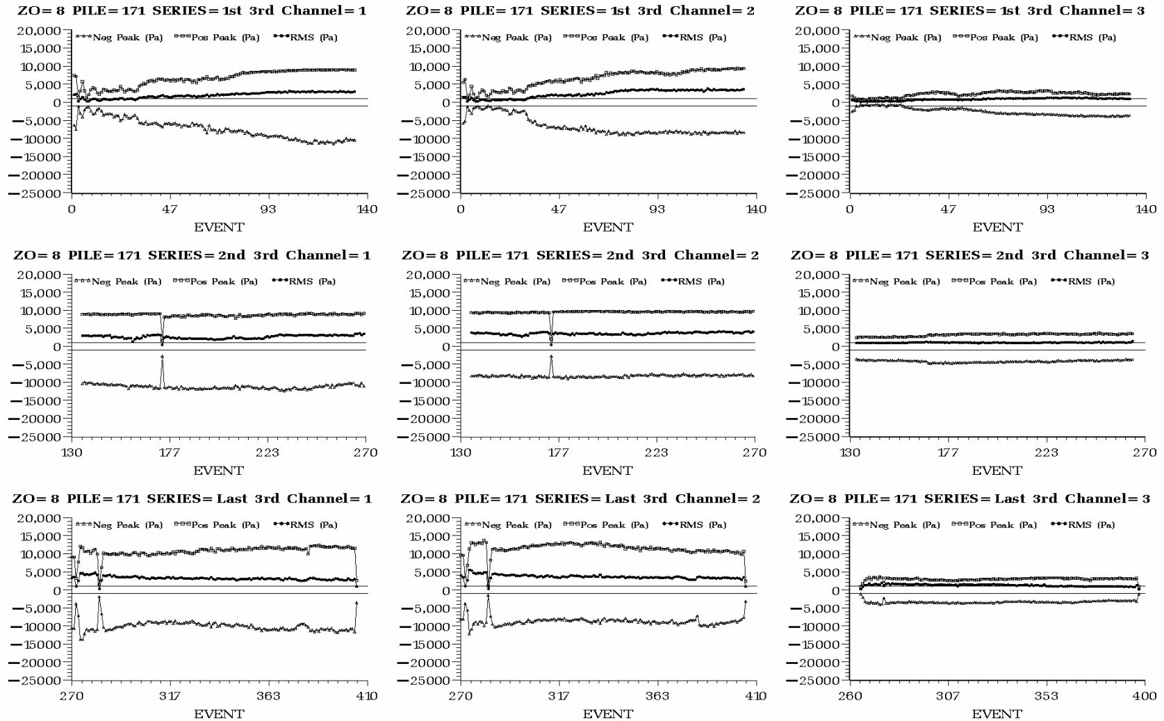
Figure C.8. Peak Positive, Peak Negative, and Root Mean Square Sound Pressure (Pa) of Each Impact on Plumb Pile 171 Driven at Hood Canal Bridge in 18 ft of Water with a Type II Confined Bubble Curtain in Place. Plots are arranged by hydrophone H1 (left) to H3 (right) and by impact series, each containing one third of the impacts, from first third (top) to last third (bottom).
