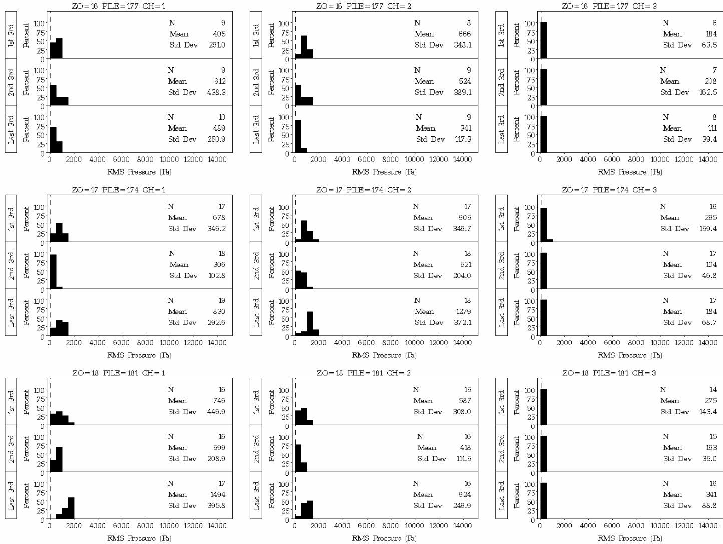
Figure D.6. Plots of Distribution Statistics on Root Mean Square Pressure for Impacts on Batter Piles 177, 174, and 181 at the Hood Canal Bridge in 37 ft, 29 ft, and 33 ft of Water, Respectively, with Type I Unconfined Bubble Curtain in Place
