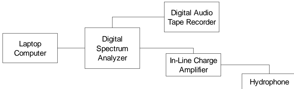
Figure 5. Diagram of Hydroacoustic Monitoring System
