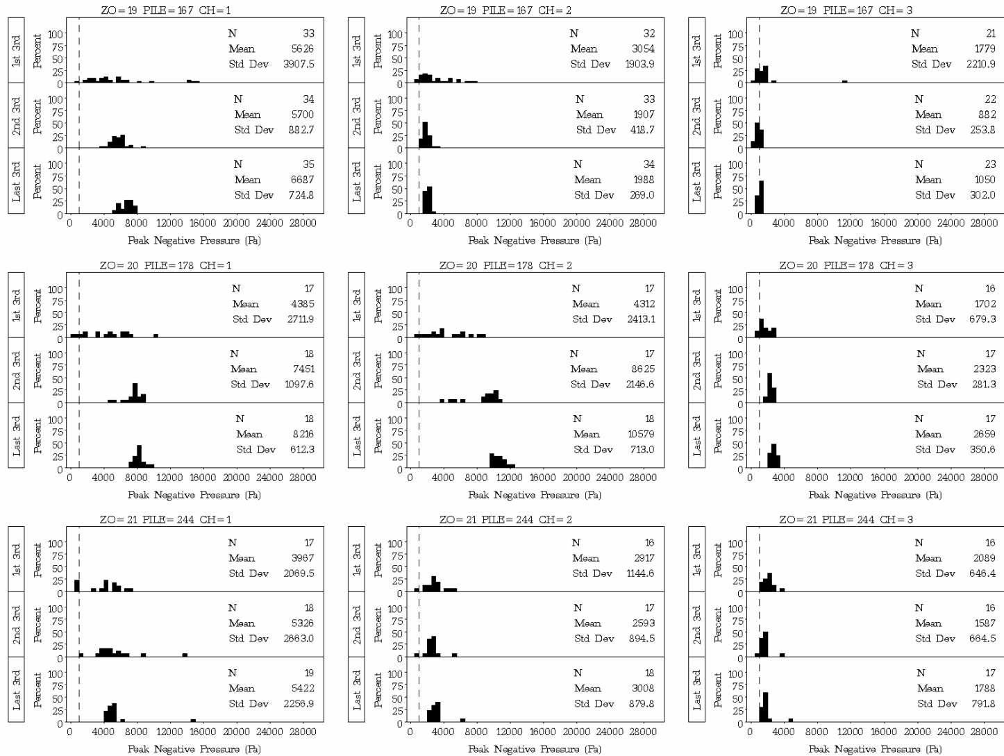
Figure D.21. Plots of Distribution Statistics on Peak Negative Pressure for Impacts on Batter Piles 167, 178, and 244 at the Hood Canal Bridge. Batter pile 167 is in 7 ft of water with a Type I unconfined bubble curtain in place; batter piles 178 and 244 are in 37 ft and 20 ft of water, respectively, with no bubble curtains in place.
