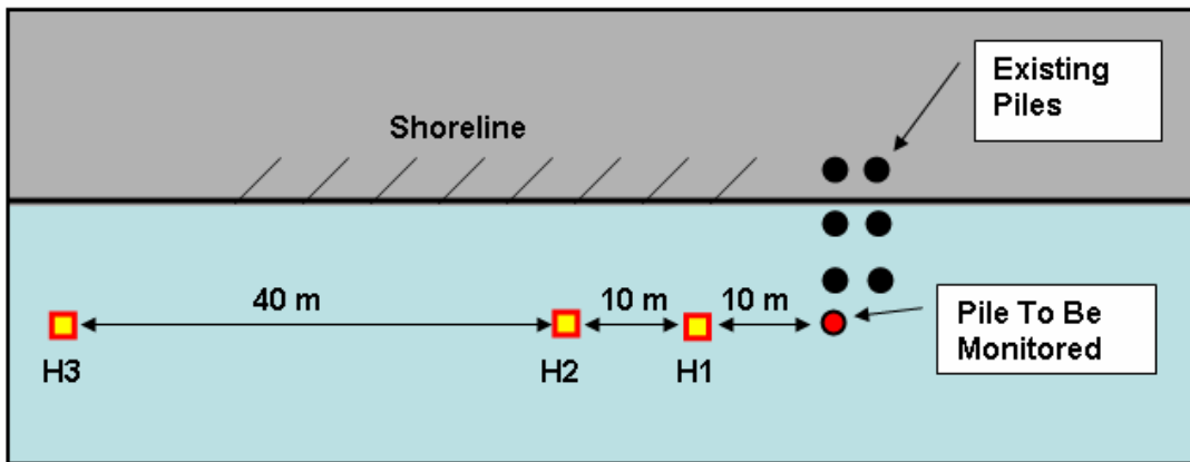
Figure 6. Schematic Plan View of Hydrophone Array
