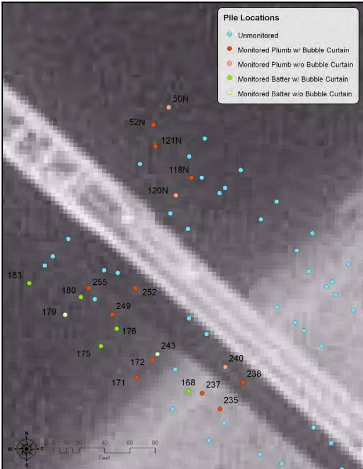
Figure 8. Locations of Plumb and Batter Piles Monitored With or Without Sound Mitigation (Bubble Curtain) During Hydroacoustic Monitoring Study, Eastern Approach of the Hood Canal Bridge
