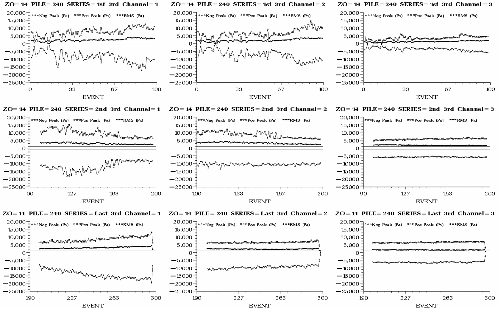
Figure C.14. Peak Positive, Peak Negative, and Root Mean Square Sound Pressure (Pa) of Each Impact on Plumb Pile 240 Driven at Hood Canal Bridge in 9 ft of Water with No Bubble Curtain in Place. Plots are arranged by hydrophone H1 (left) to H3 (right) and by impact series, each containing one third of the impacts, from first third (top) to last third (bottom).
