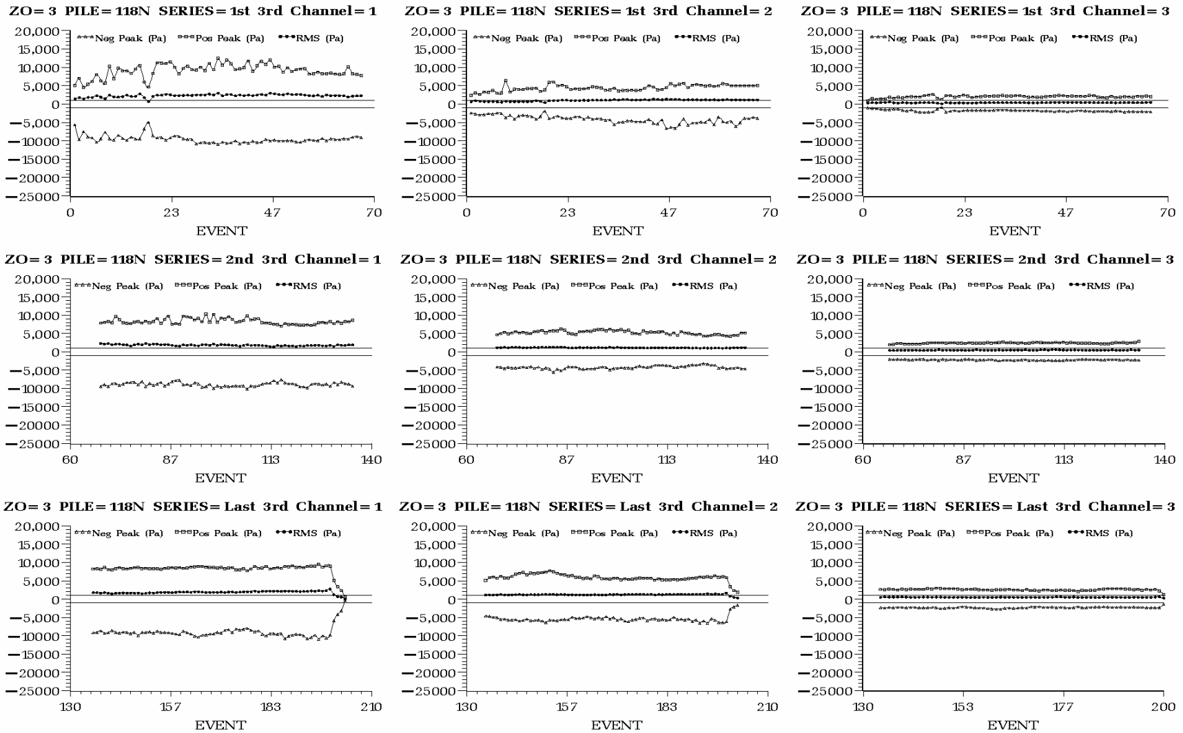
Figure C.3. Peak Positive, Peak Negative, and Root Mean Square Sound Pressure (Pa) of Each Impact at Plumb Pile 118N Driven in 39 ft of Water with Type II Confined Bubble Curtain in Place. Plots are arranged by hydrophone H1 (left) to H3 (right) and by impact series, each containing one third of the impacts, from first third (top) to last third (bottom).
