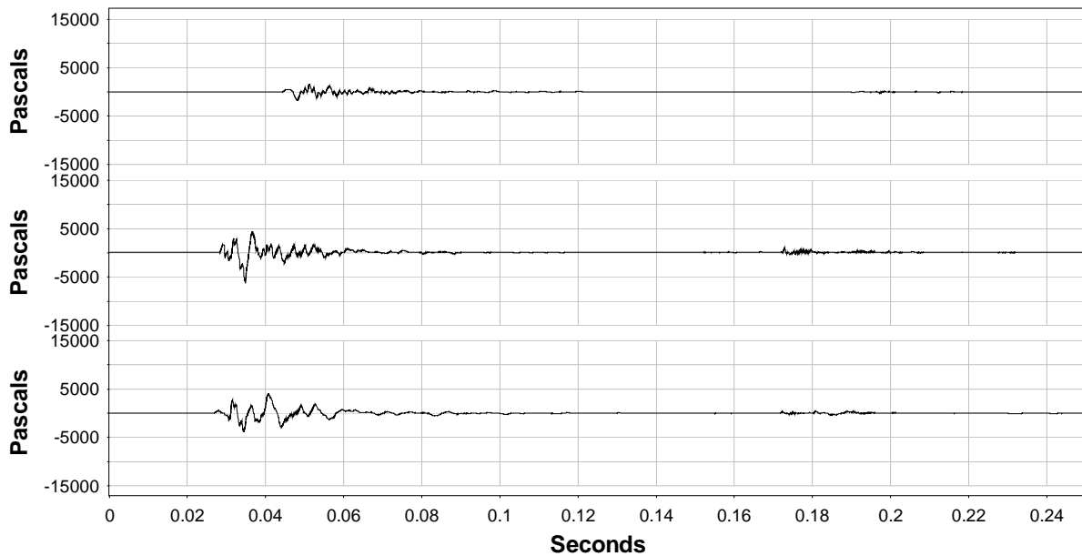
Figure 10. Sound-Pressure Levels Measured for a Single Impact of Batter Pile 178 Driven in 37 ft of Water without Bubble Curtain in Place (bottom, H1; middle, H2; top, H3)
