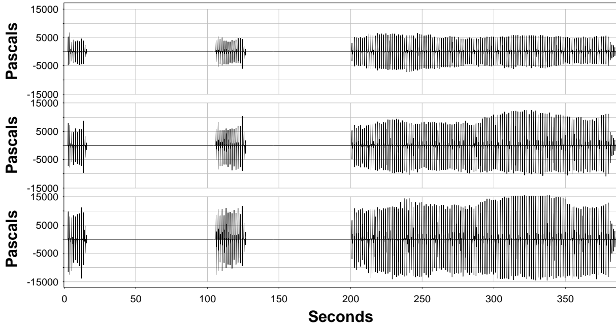
Figure A.13. Sound-Pressure Levels (Pa) Measured for Plumb Pile 120N Driven in 39 ft of Water with No Bubble Curtain.
