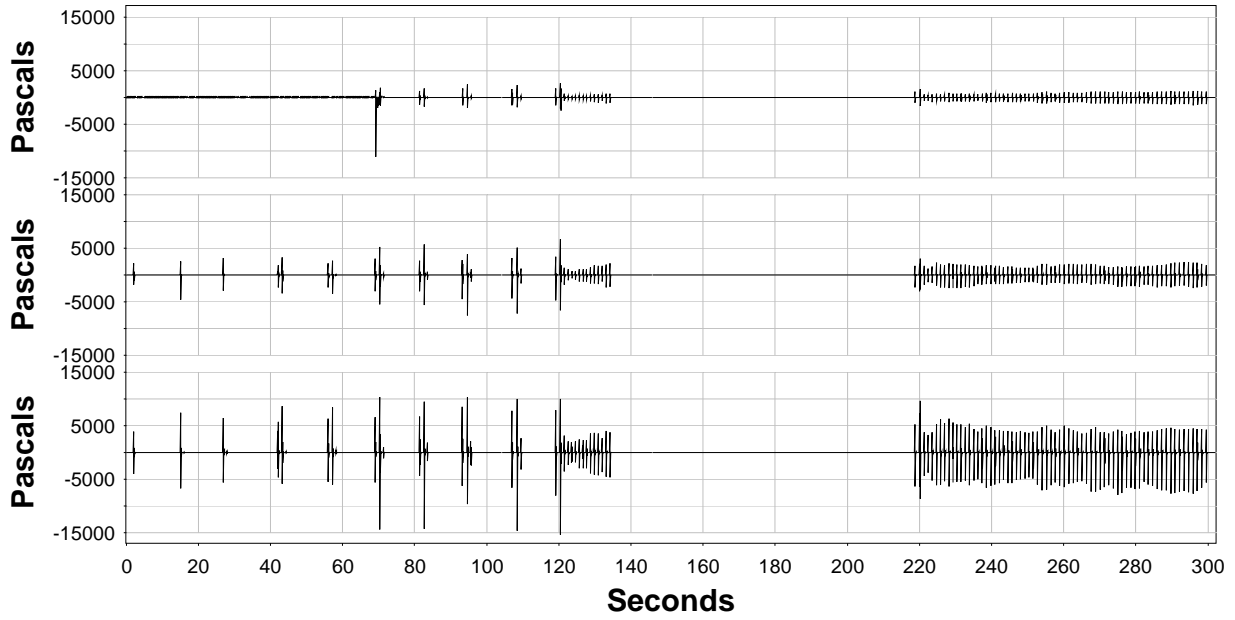
Figure A.19. Sound-Pressure Levels (Pa) Measured for Batter Pile 167 Driven in 7 ft of Water with the Bubble Curtain in Place.
