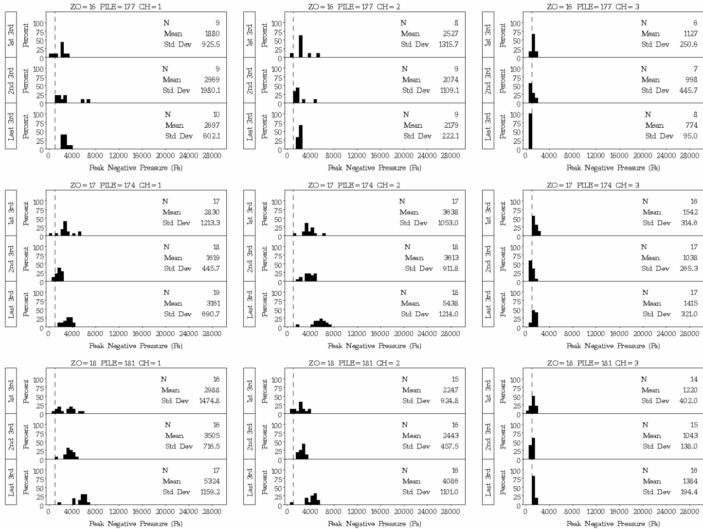
Figure D.20. Plots of Distribution Statistics on Peak Negative Pressure for Impacts on Batter Piles 177, 174, and 181 at the Hood Canal Bridge in 37 ft, 29 ft, and 33 ft of Water, Respectively, with Type I Unconfined Bubble Curtain in Place
