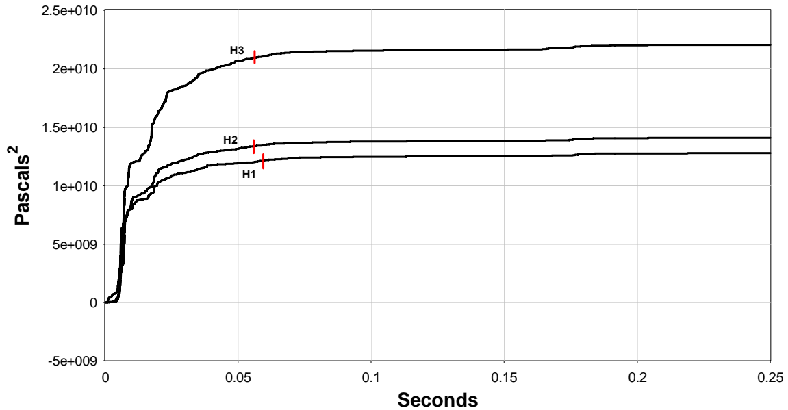
Figure 17. Power Spectral Density Indices (Figure 17a: H1 top plot, H2 middle plot, H3 bottom plot) and Cumulative Sound Exposure Over Time (Figure 17b) for a Single Pile-Driving Impact Measured at Plumb Pile 50N, Driven in 40 ft of Water Without Bubble Curtain. On the cumulative sound plot, the vertical lines represent the point in time when the summed squared sound pressures of the waveform total 95% of the sound energy.
