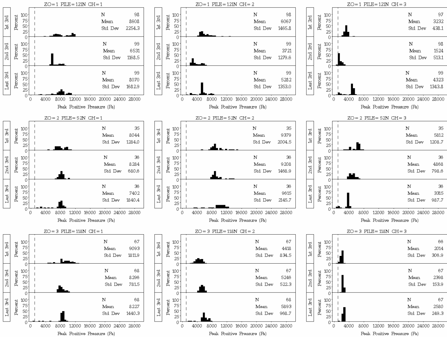
Figure D.8. Plots of Distribution Statistics on Peak Positive Pressure for Impacts on Plumb Piles 121N, 52N, and 118N at the Hood Canal Bridge in 42 ft, 40 ft, and 39 ft of Water, Respectively, with Type II Confined Bubble Curtain in Place
