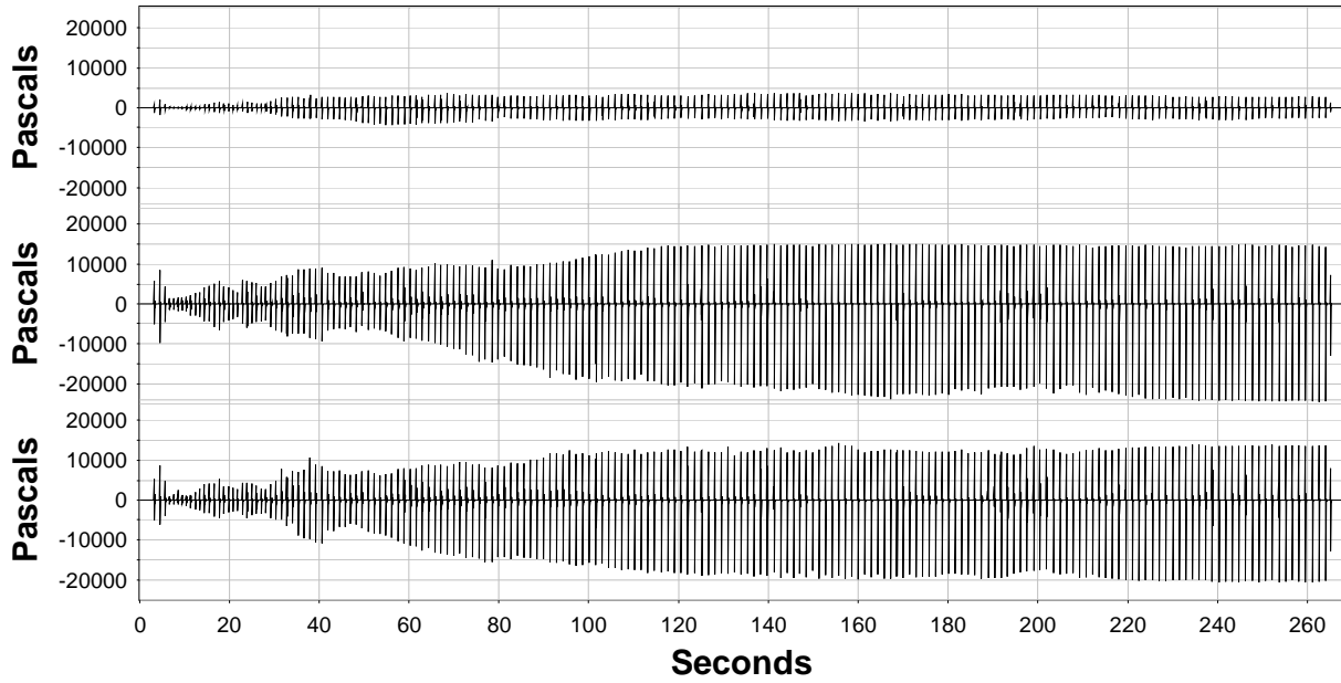
Figure A.7. Sound-Pressure Levels (Pa) Measured for Plumb Pile 172 Driven in 20 ft of Water with the Bubble Curtain in Place.
