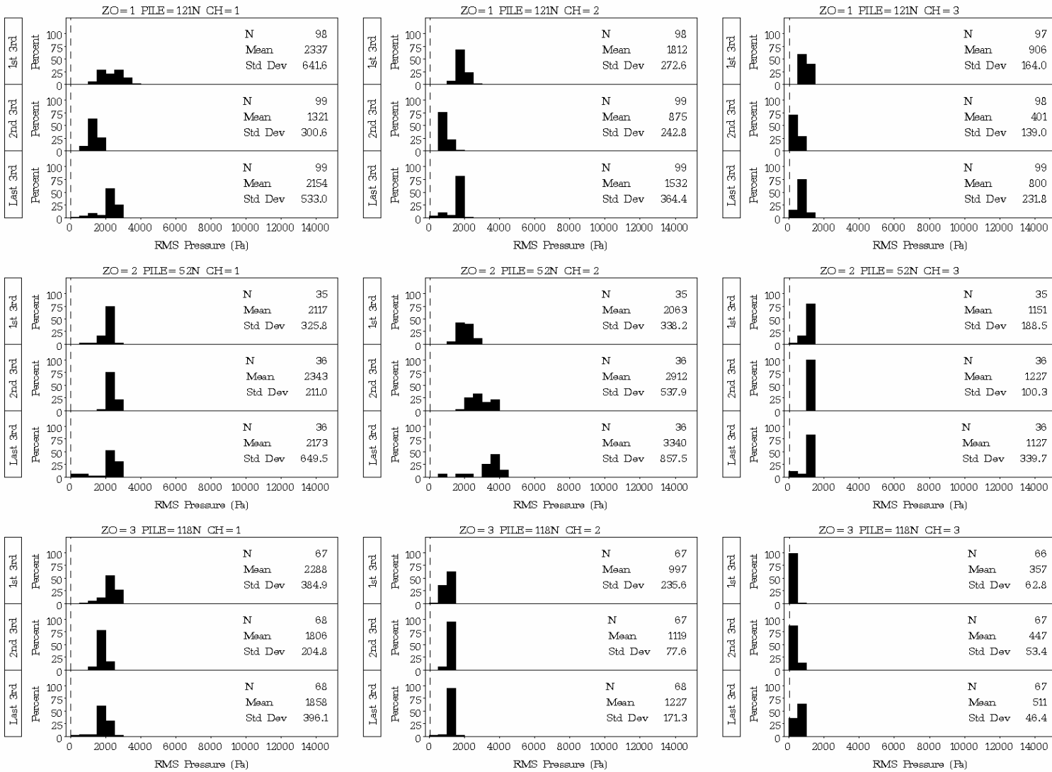
Figure D.1. Plots of Distribution Statistics on Root Mean Square Pressure for Impacts on Plumb Piles 121N, 52N, and 118N at the Hood Canal Bridge in 42 ft, 40 ft, and 39 ft of Water, Respectively, with Type II Confined Bubble Curtain in Place
