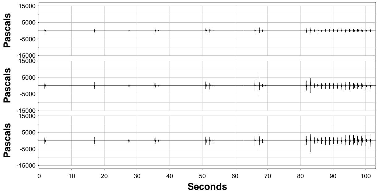
Figure A.16. Sound-Pressure Levels (Pa) Measured for Batter Pile 177 Driven in 37 ft of Water with the Bubble Curtain in Place.
