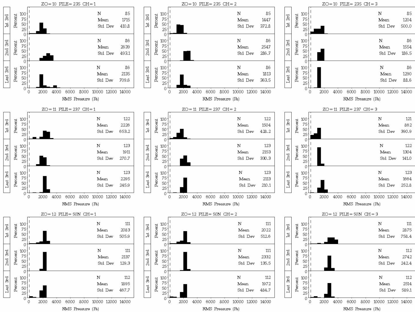
Figure D.4. Plots of Distribution Statistics on Root Mean Square Pressure for Impacts on Plumb Piles 235 and 237 in 4.5 ft and 4 ft of Water, Respectively, with a Type II Confined Bubble Curtain in Place, and at Plumb Pile 50N in 40 ft of Water with No Bubble Curtain in Place
