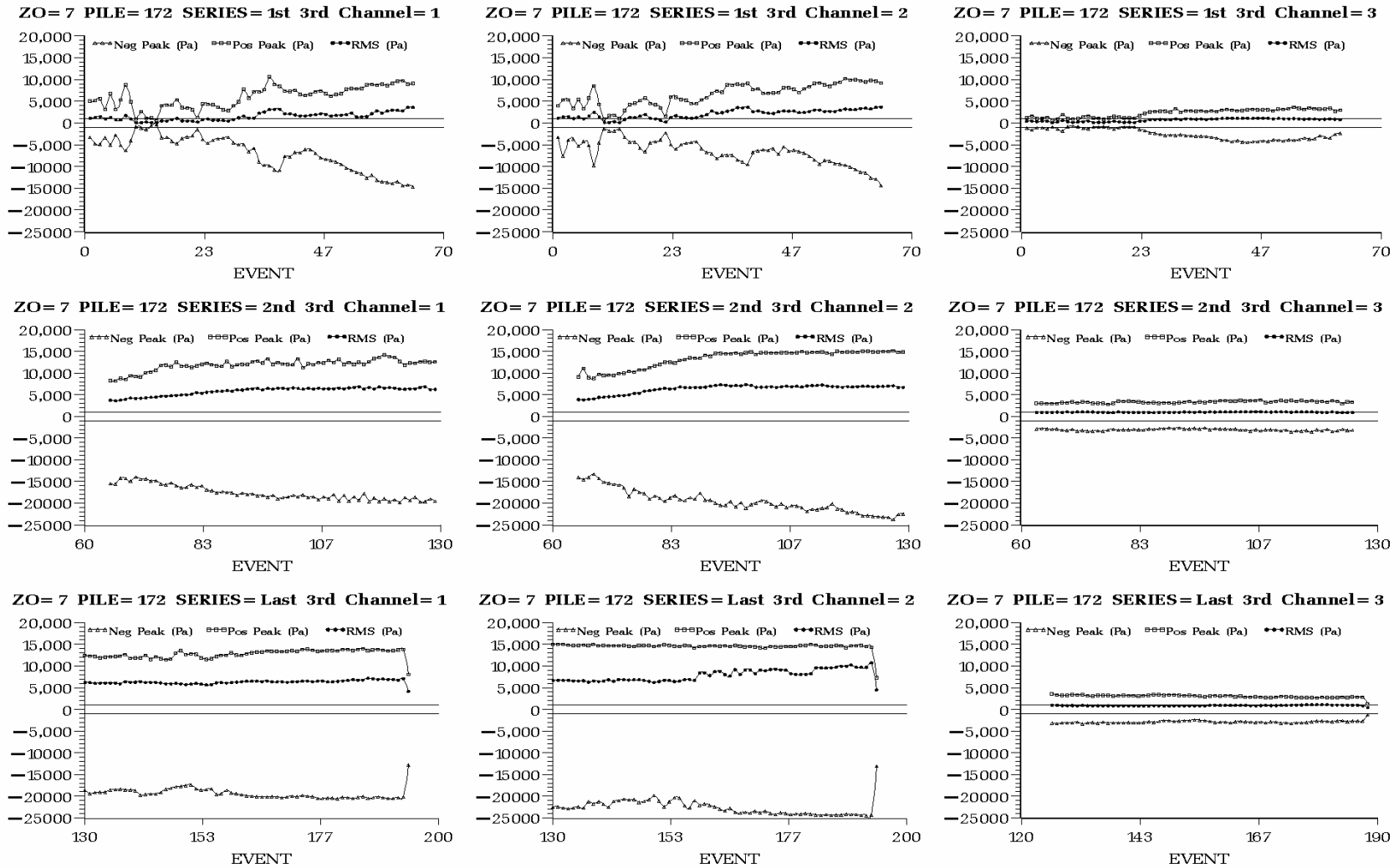
Figure C.7. Peak Positive, Peak Negative, and Root Mean Square Sound Pressure (Pa) of Each Impact on Plumb Pile 172 Driven at Hood Canal Bridge in 20 ft of Water with a Type II Confined Bubble Curtain in Place. Plots are arranged by hydrophone H1 (left) to H3 (right) and by impact series, each containing one third of the impacts, from first third (top) to last third (bottom).
