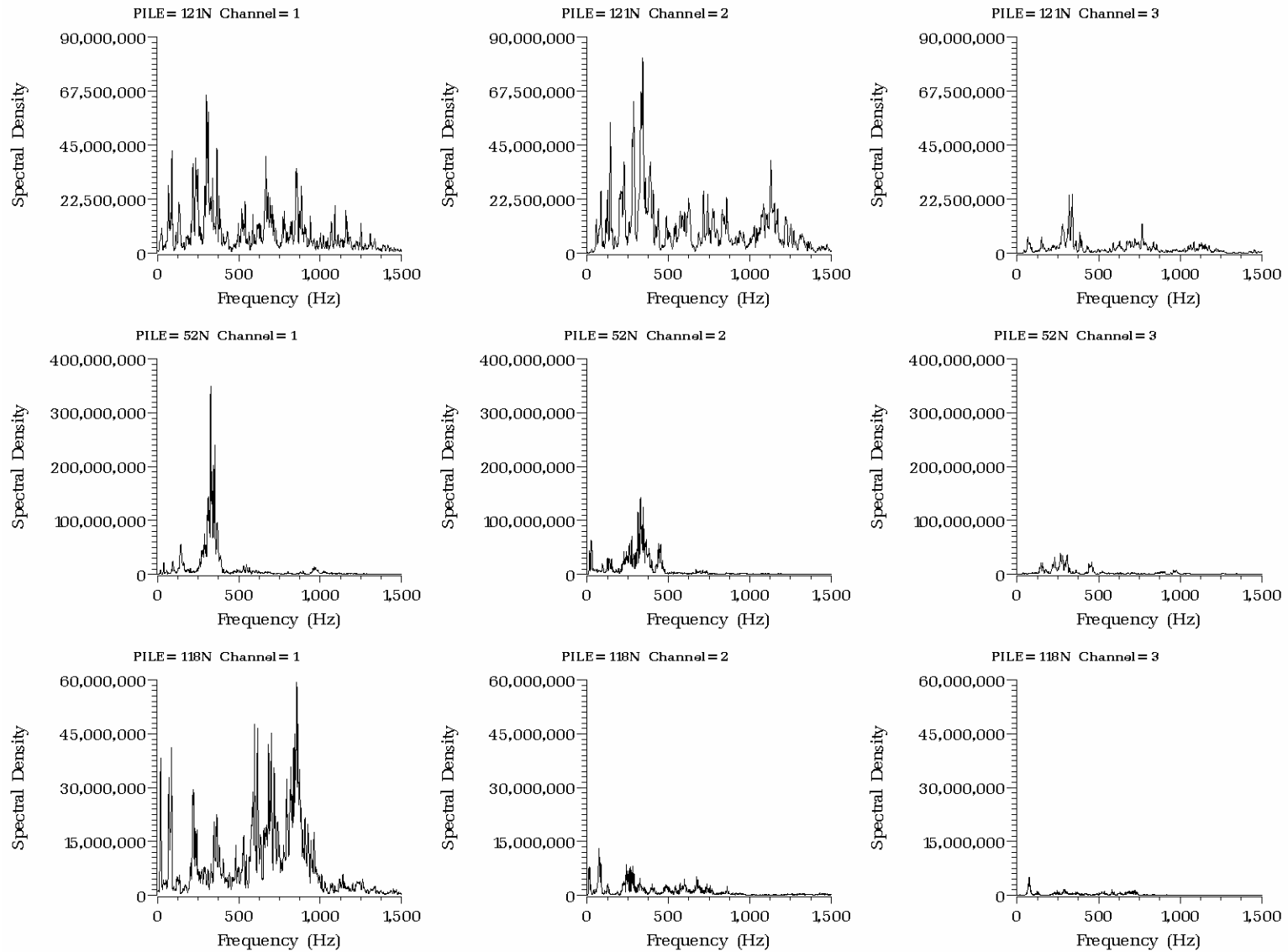
Figure E.1. Spectral Density ( \text{Pa}^2/\text{Hz} ) Versus Frequency (Hz) at Hydrophones H1 (left), H2 (center), and H3 (right) for the First 20 Impacts on Piles 121N, 52N, and 118N (all plumb piles driven with Type II confined bubble curtain in place)
