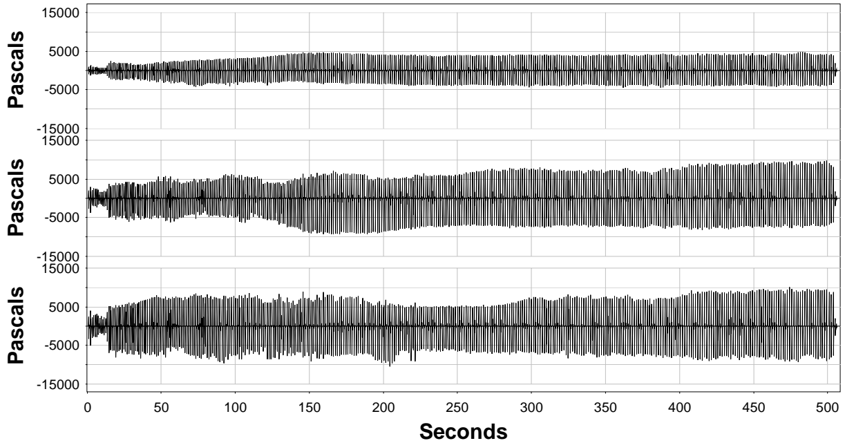
Figure A.11. Sound-Pressure Levels (Pa) Measured for Plumb Pile 237 Driven in 4 ft of Water with the Bubble Curtain in Place.
