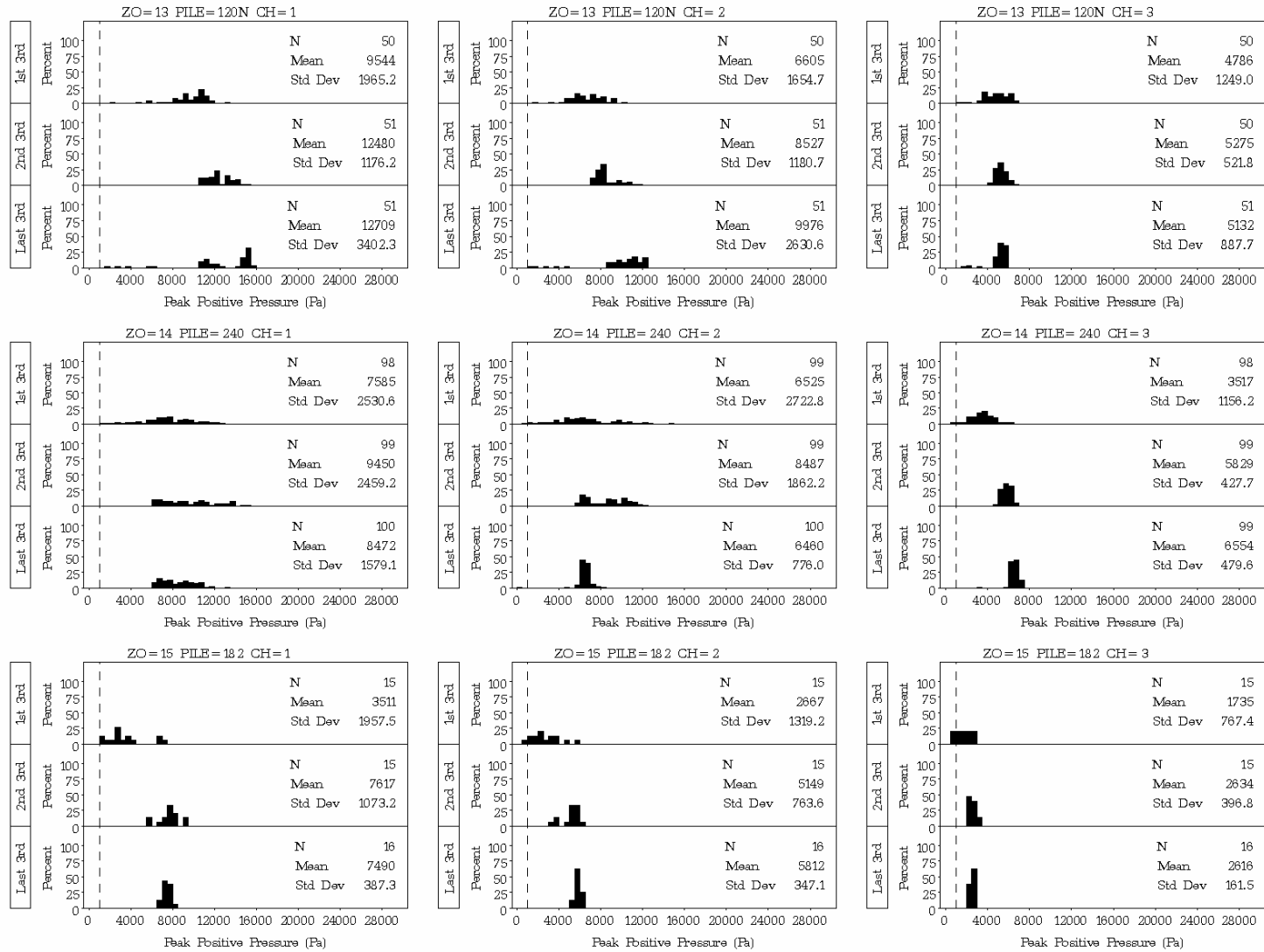
Figure D.12. Plots of Distribution Statistics on Peak Positive Pressure for Impacts on Plumb Piles 120N and 240 in 39 ft and 9 ft of Water, Respectively, with No Bubble Curtain in Place, and on Batter Pile 182 in 41 ft of Water with No Bubble Curtain in Place
