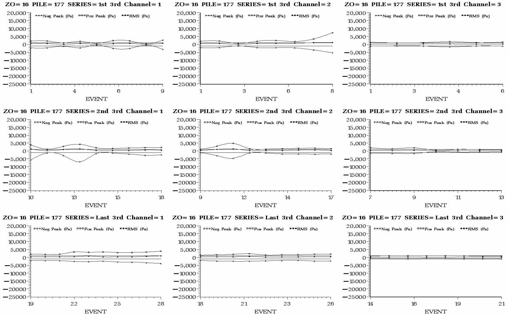
Figure C.16. Peak Positive, Peak Negative, and Root Mean Square Sound Pressure (Pa) of Each Impact on Batter Pile 177 Driven at Hood Canal Bridge in 37 ft of Water with a Type I Unconfined Bubble Curtain in Place. Plots are arranged by hydrophone H1 (left) to H3 (right) and by impact series, each containing one third of the impacts, from first third (top) to last third (bottom).
