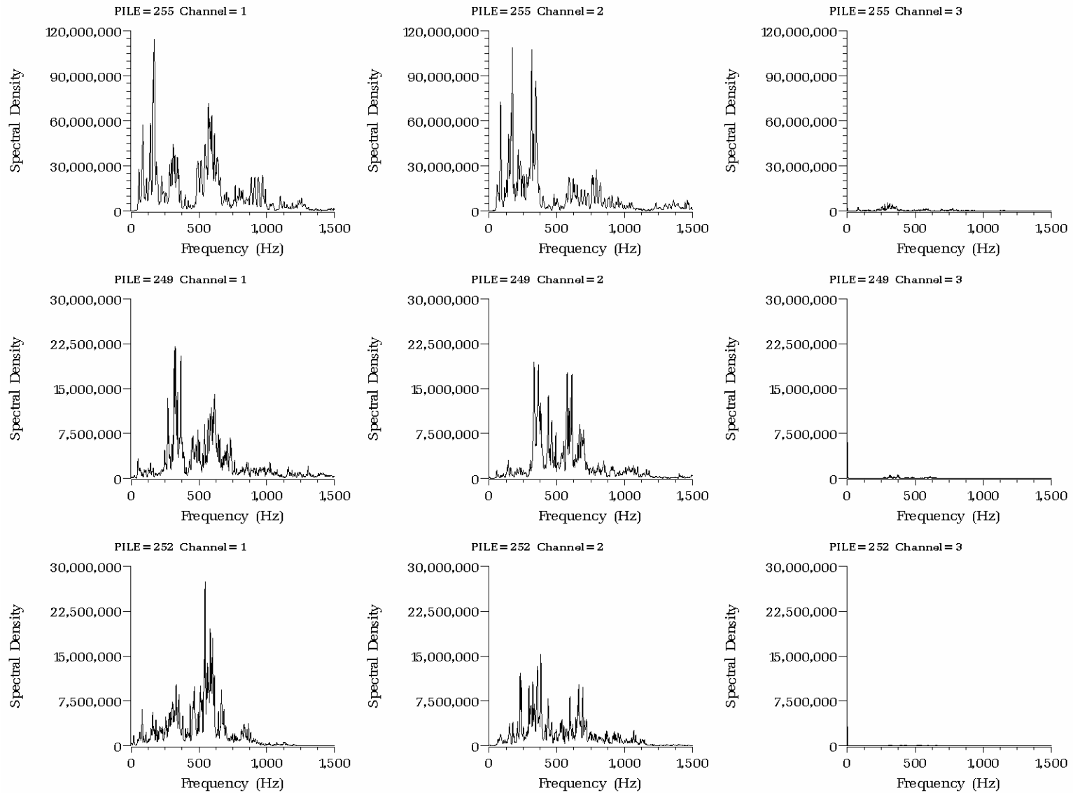
Figure E.2. Spectral Density (Pa 2 /Hz) Versus Frequency (Hz) at Hydrophones H1 (left), H2 (center), and H3 (right) for the First 20 Impacts on Piles 255, 249, and 252 (all plumb piles driven with Type II confined bubble curtain in place)
