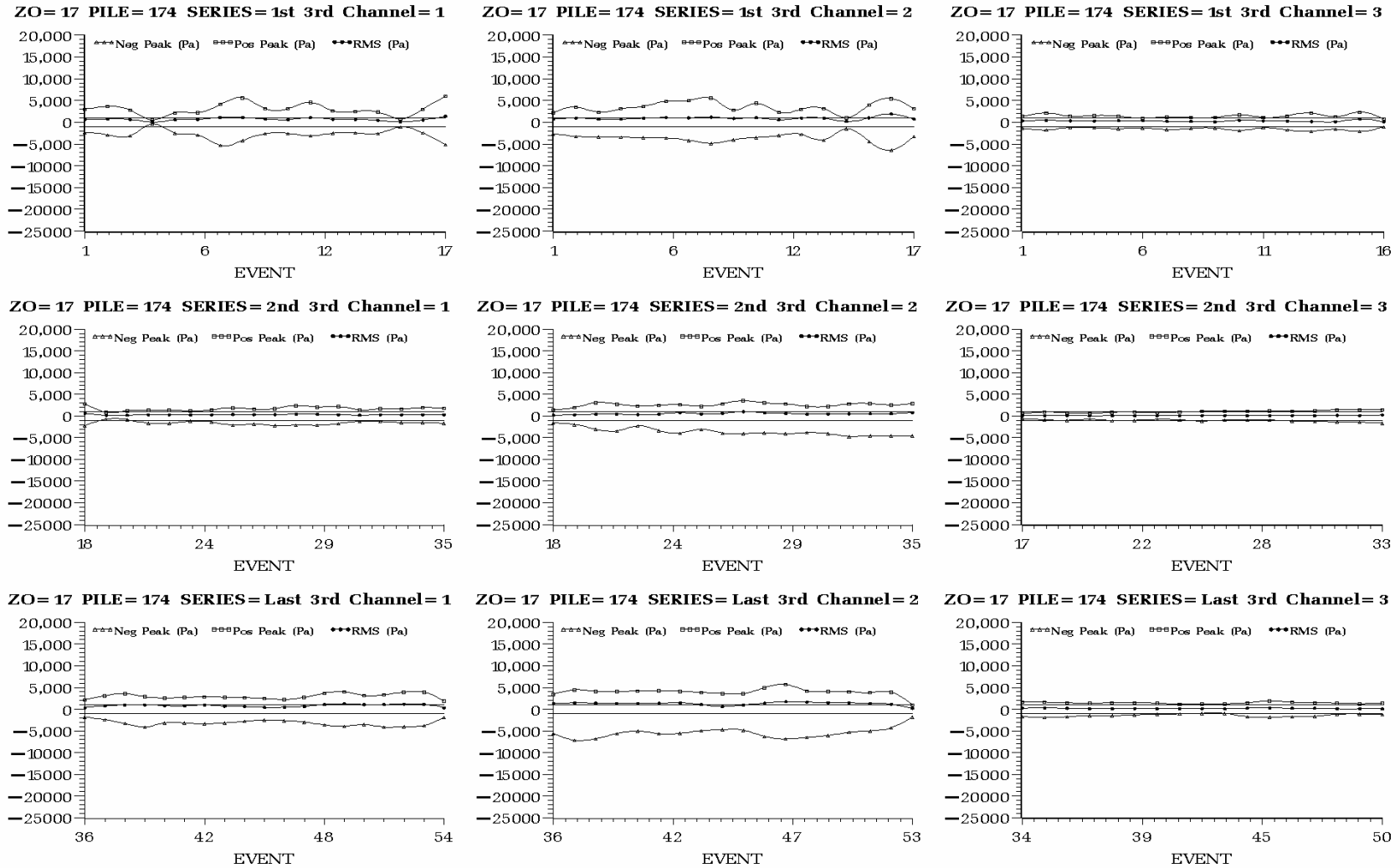
Figure C.17. Peak Positive, Peak Negative, and Root Mean Square Sound Pressure (Pa) of Each Impact on Batter Pile 174 Driven at Hood Canal Bridge in 29 ft of Water with a Type I Unconfined Bubble Curtain in Place. Plots are arranged by hydrophone H1 (left) to H3 (right) and by impact series, each containing one third of the impacts, from first third (top) to last third (bottom).
