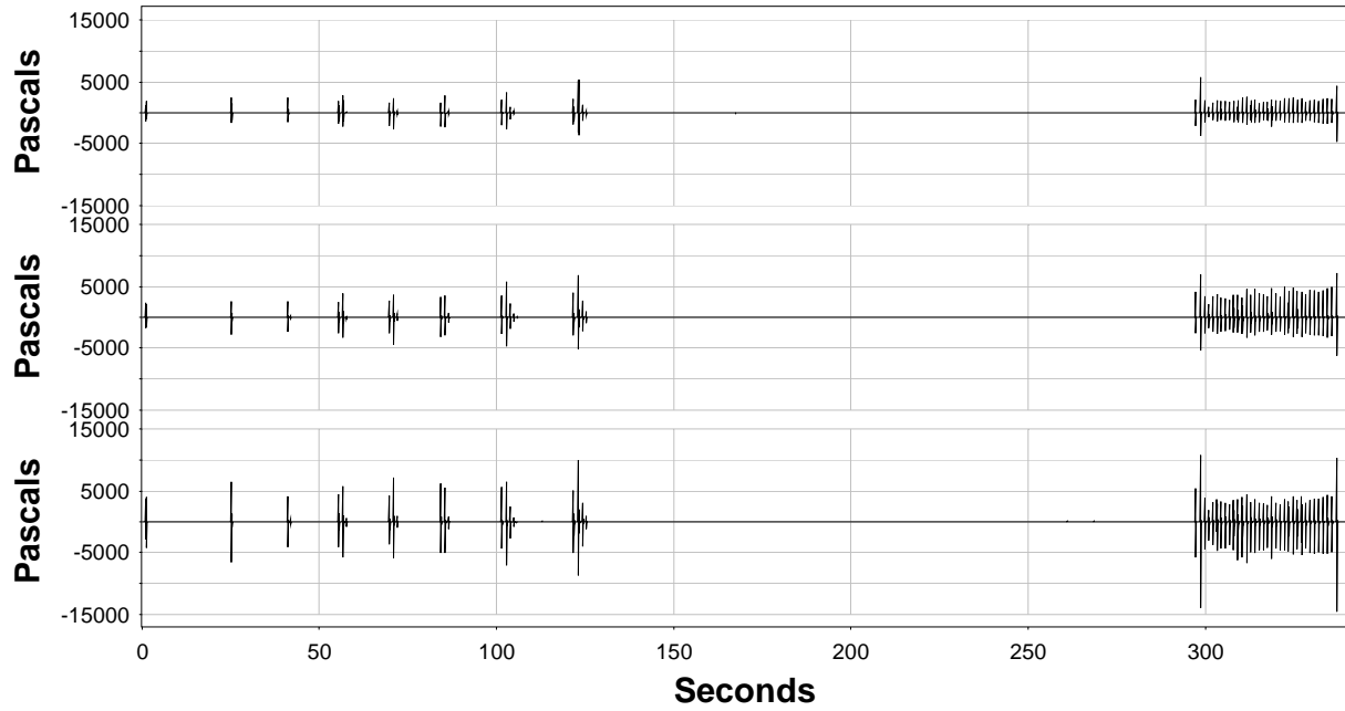
Figure A.21. Sound-Pressure Levels (Pa) Measured for Batter Pile 244 Driven in 7 ft of Water with No Bubble Curtain.
