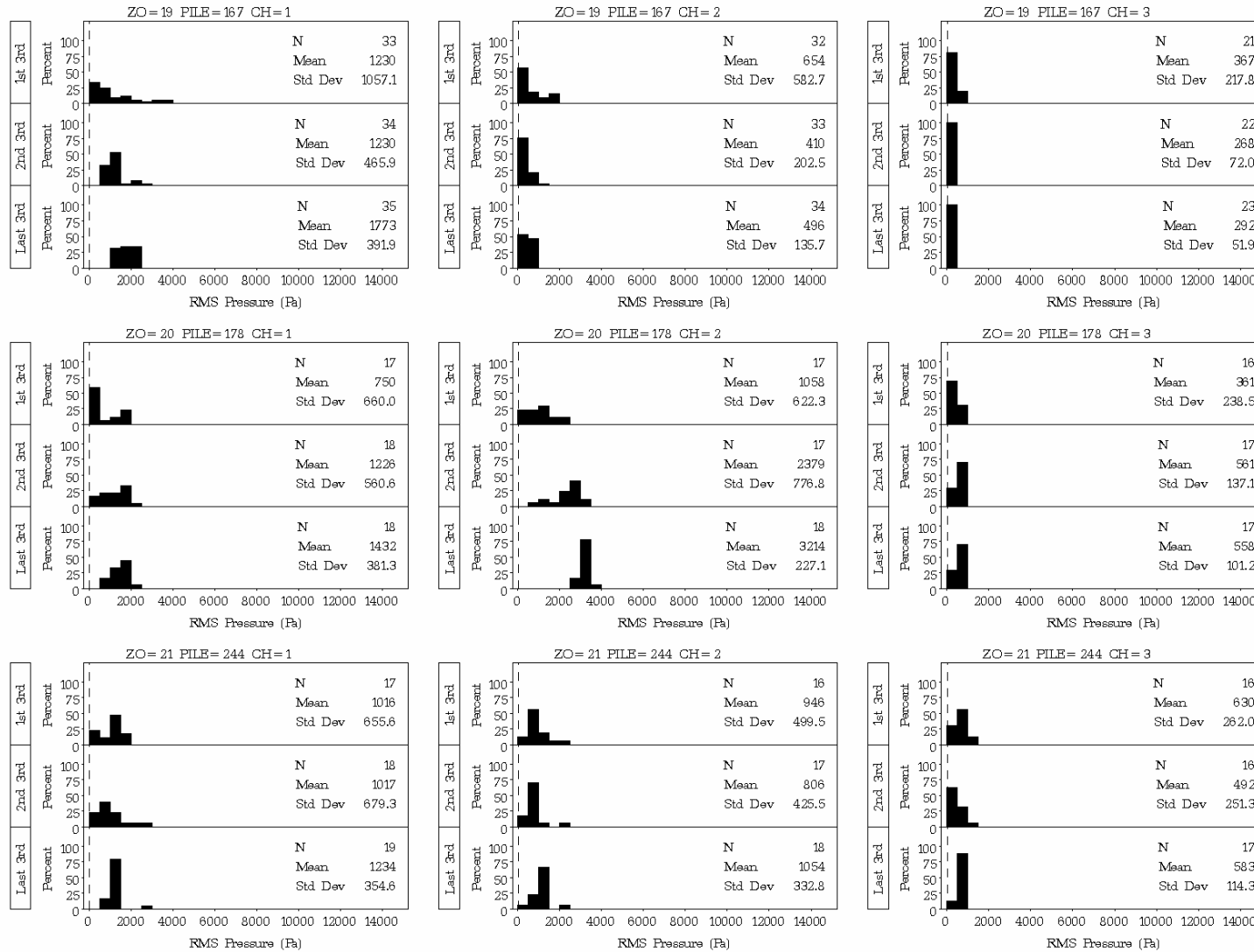
Figure D.7. Plots of Distribution Statistics on Root Mean Square Pressure for Impacts on Batter Piles 167, 178, and 244 at the Hood Canal Bridge. Batter pile 167 is in 7 ft of water with a Type I unconfined bubble curtain in place; batter piles 178 and 244 are in 37 ft and 20 ft of water, respectively, with no bubble curtains in place.
