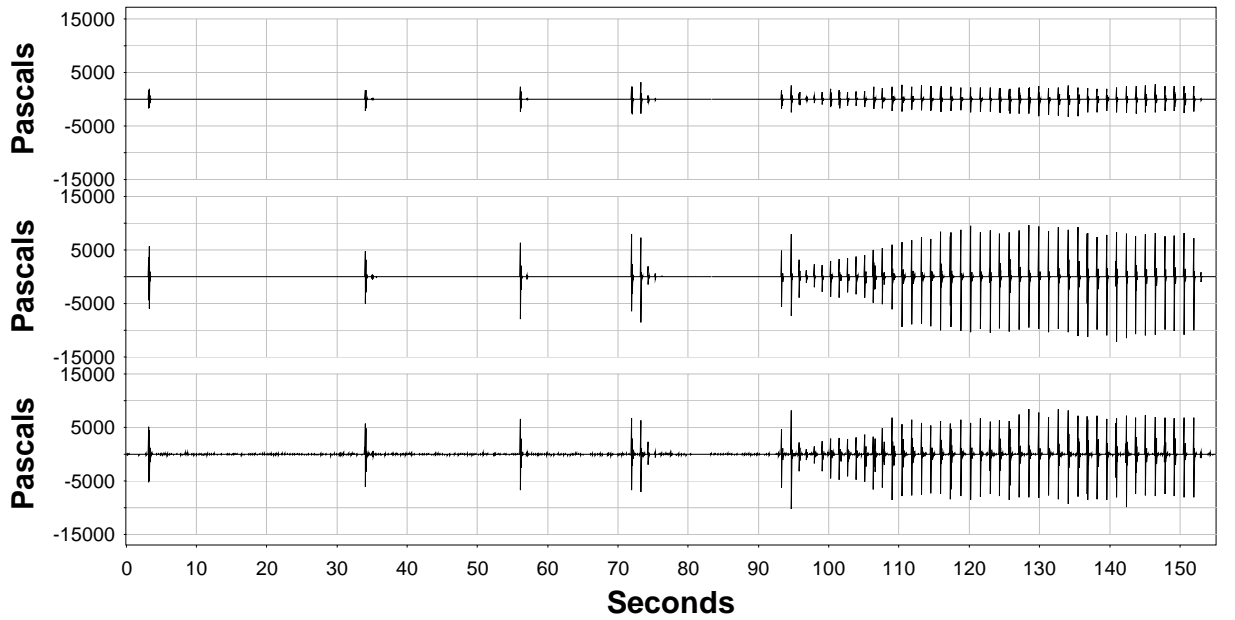
Figure A.20. Sound-Pressure Levels (Pa) Measured for Batter Pile 178 Driven in 37 ft of Water with No Bubble Curtain.
