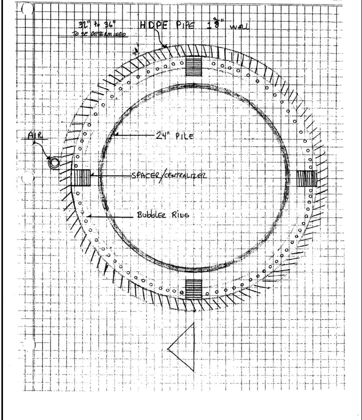
Figure F. 2. Contractor's Plan View Drawing of Bubble Ring for Confined Bubble Curtain used on Plumb Piles
