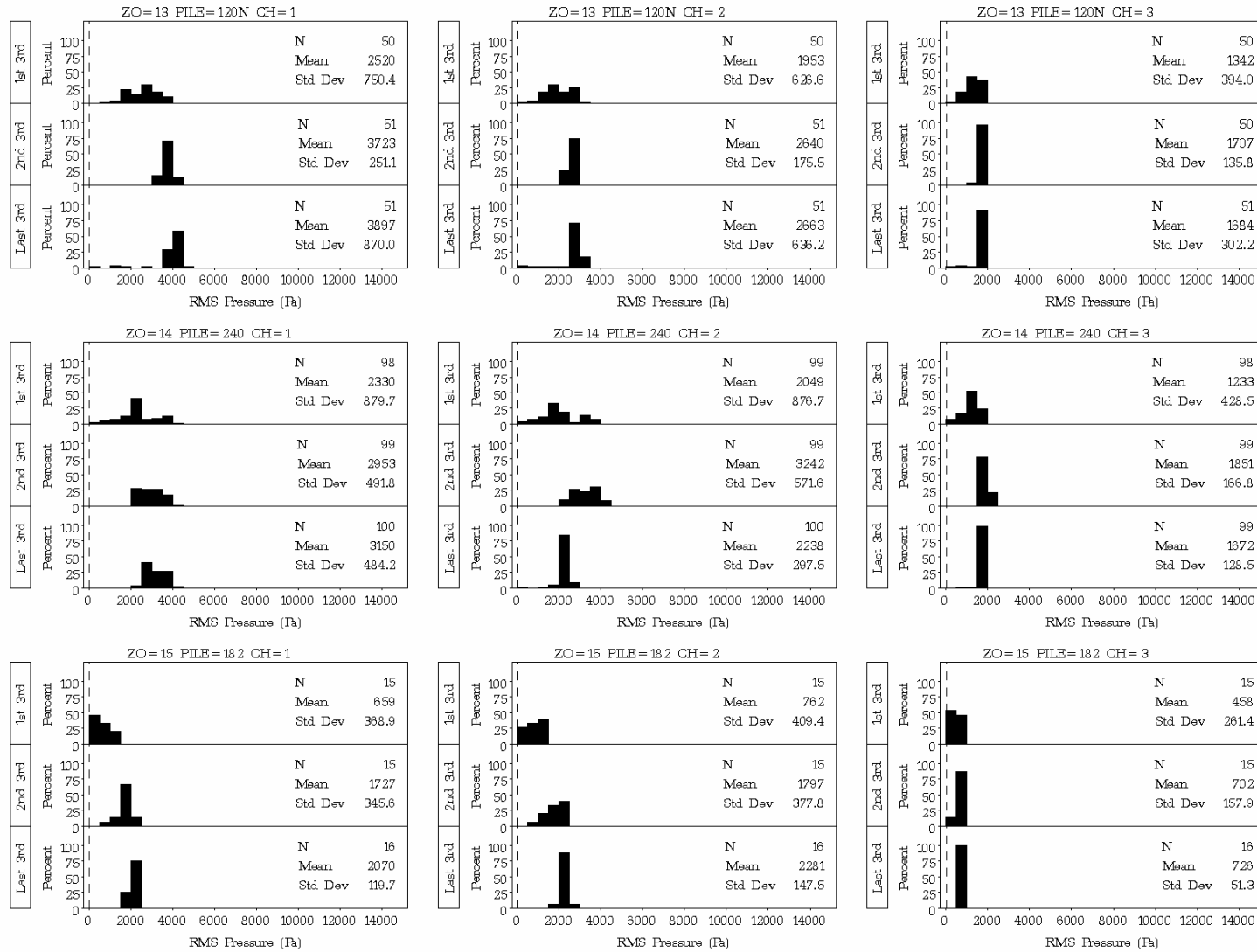
Figure D.5. Plots of Distribution Statistics on Root Mean Square Pressure for Impacts on Plumb Piles 120N and 240 in 39 ft and 9 ft of Water, Respectively, with No Bubble Curtain in Place, and on Batter Pile 182 in 41 ft of Water with No Bubble Curtain in Place
