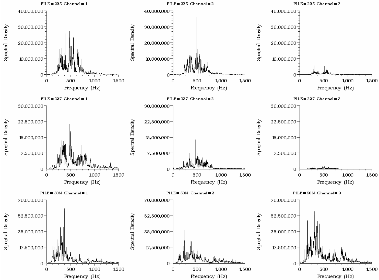
Figure E.4. Spectral Density (Pa 2 /Hz) Versus Frequency (Hz) at Hydrophones H1 (left), H2 (center), and H3 (right) for the First 20 Impacts on Piles 235, 237 (plumb piles driven with Type II confined bubble curtain in place), and 50N (plumb pile driven without bubble curtain)
