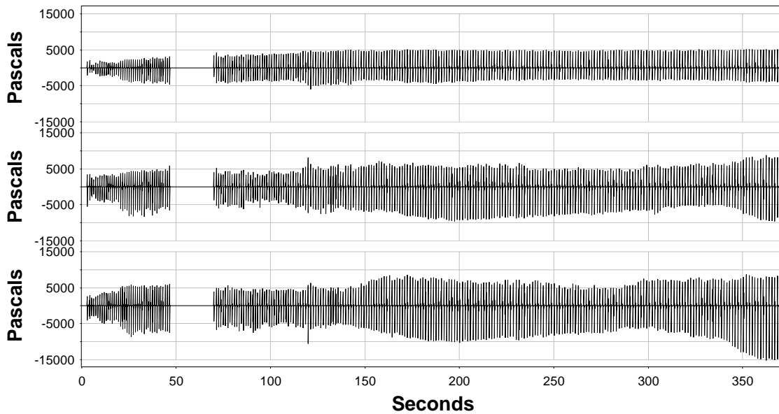
Figure 13. Sound-Pressure Levels (Pa) Measured for Plumb Pile 235 Driven in 4.5 ft of Water with the Bubble Curtain in Place. H1 (bottom plot), H2 (middle plot), and H3 (top plot) were approximately 64.7, 89.1, and 154.8 ft from the pile, respectively.
