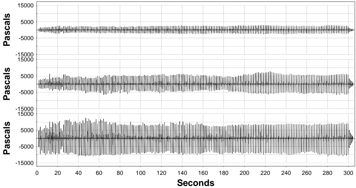
Figure A.3. Sound-Pressure Levels (Pa) Measured for Plumb Pile 118N Driven in 39 ft of Water with the Bubble Curtain in Place.
