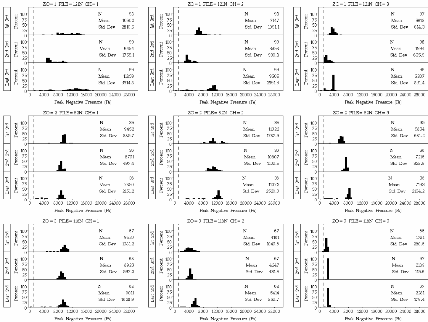
Figure D.15. Plots of Distribution Statistics on Peak Negative Pressure for Impacts on Plumb Piles 121N, 52N, and 118N at the Hood Canal Bridge in 42 ft, 40 ft, and 39 ft of Water, Respectively, with Type II Confined Bubble Curtain in Place
