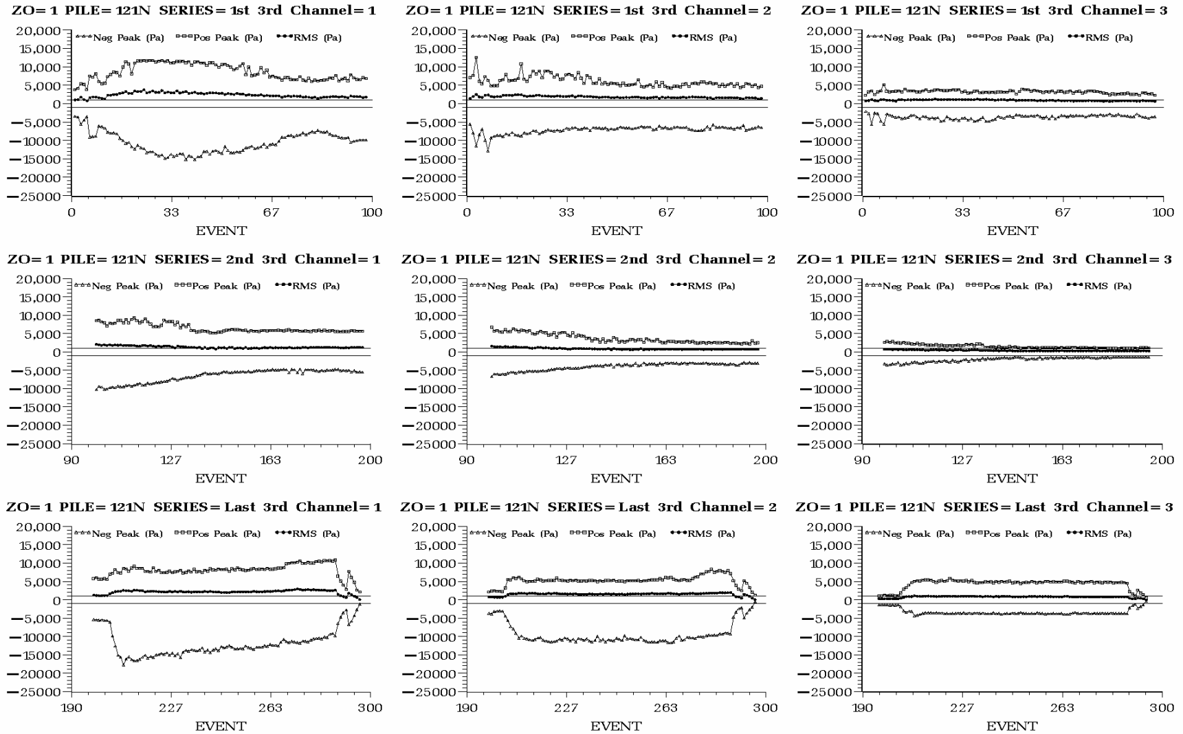
Figure C.1. Peak Positive, Peak Negative, and Root Mean Square Sound Pressure (Pa) of Each Impact at Plumb Pile 121N Driven in 42 ft Water with a Type II Confined Bubble Curtain in Place. Plots are arranged by hydrophone H1 (left) to H3 (right) and by impact series, each containing one third of the impacts, from first third (top) to last third (bottom).
