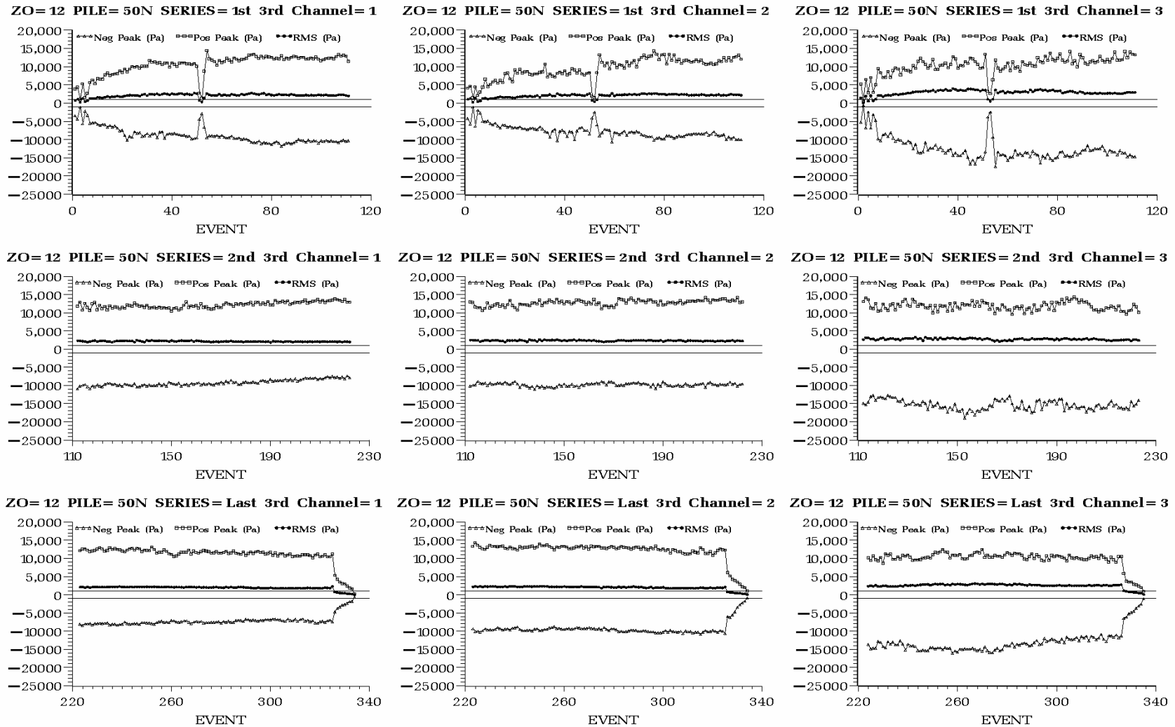
Figure C.12. Peak Positive, Peak Negative, and Root Mean Square Sound Pressure (Pa) of Each Impact on Plumb Pile 50N Driven at Hood Canal Bridge in 40 ft of Water with No Bubble Curtain in Place. Plots are arranged by hydrophone H1 (left) to H3 (right) and by impact series, each containing one third of the impacts, from first third (top) to last third (bottom).
