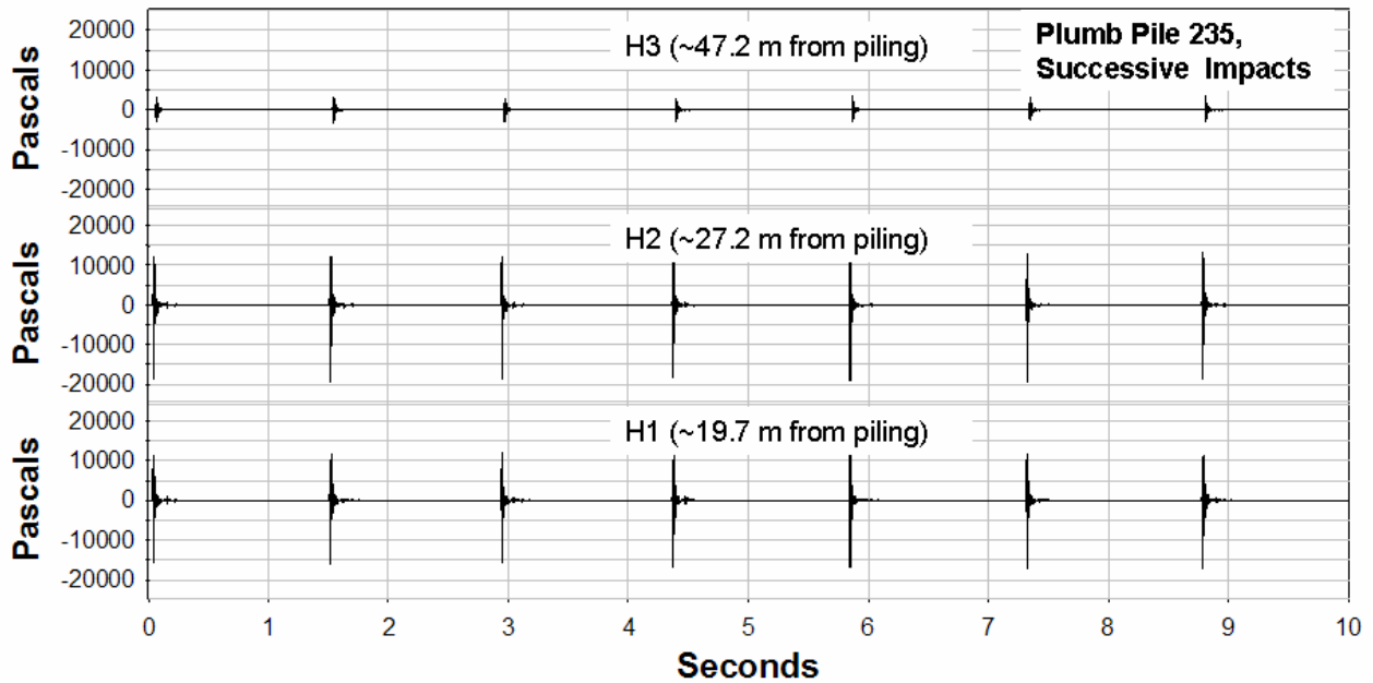
Figure 11. Sound-Pressure Levels Measured over Successive Impacts for Plumb Pile 235 Driven in 4.5 ft of Water with the Bubble Curtain in Place (bottom, H1; middle, H2; top, H3)
