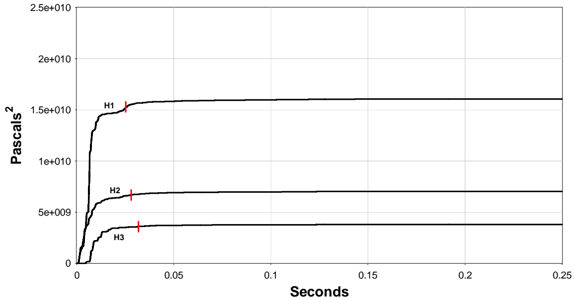
Figure 19. Power Spectral Density Indices (Figure 19a: H1 top plot, H2 middle plot, H3 bottom plot) and Cumulative Sound Exposure Over Time (Figure 19b) for a Single Pile-Driving Impact Measured at Plumb Pile 240, Driven in 9 ft of Water Without Bubble Curtain. On the cumulative sound plot, the vertical lines represent the point in time when the summed squared sound pressures of the waveform total 95% of the sound energy.
