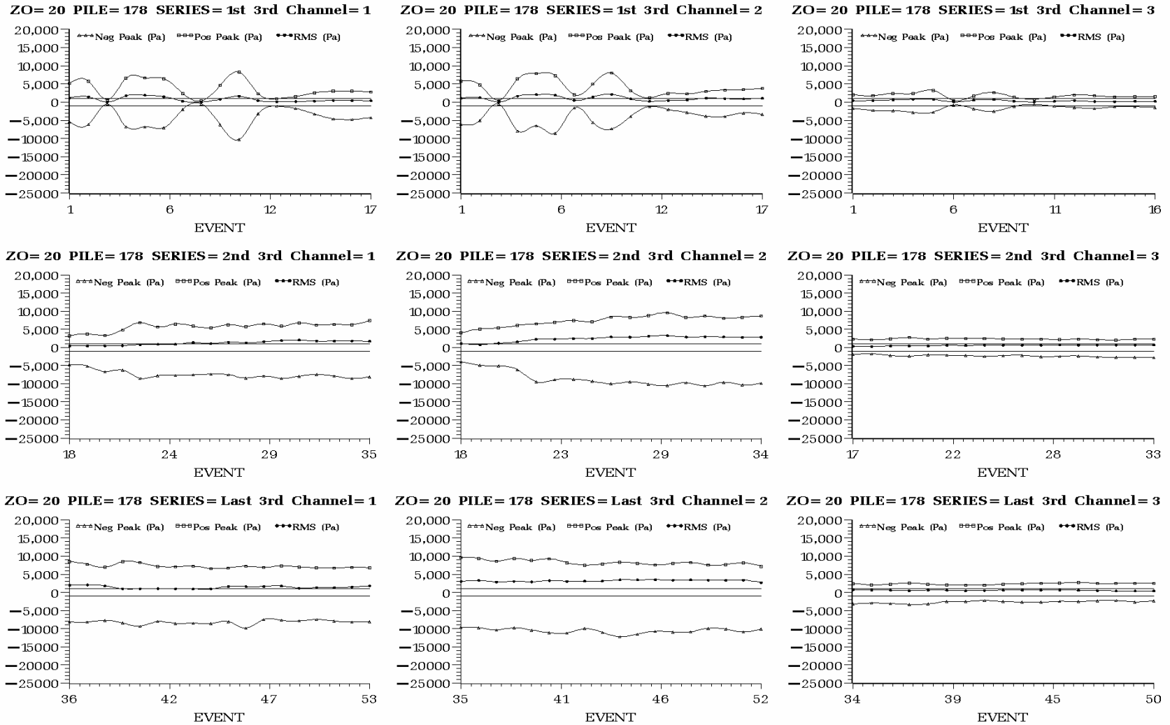
Figure C.20. Peak Positive, Peak Negative, and Root Mean Square Sound Pressure (Pa) of Each Impact on Batter Pile 178 Driven at Hood Canal Bridge in 37 ft of Water with No Bubble Curtain in Place. Plots are arranged by hydrophone H1 (left) to H3 (right) and by impact series, each containing one third of the impacts, from first third (top) to last third (bottom).
