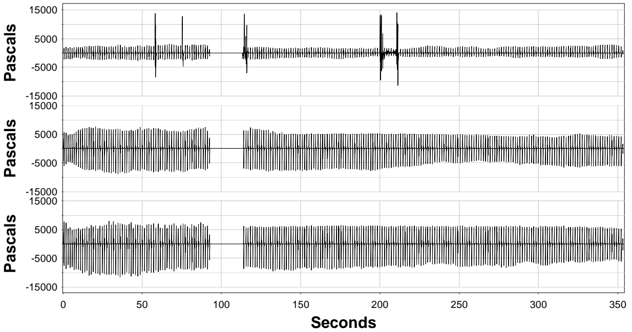
Figure A.4. Sound-Pressure Levels (Pa) Measured for Plumb Pile 255 Driven in 33 ft of Water with the Bubble Curtain in Place.
