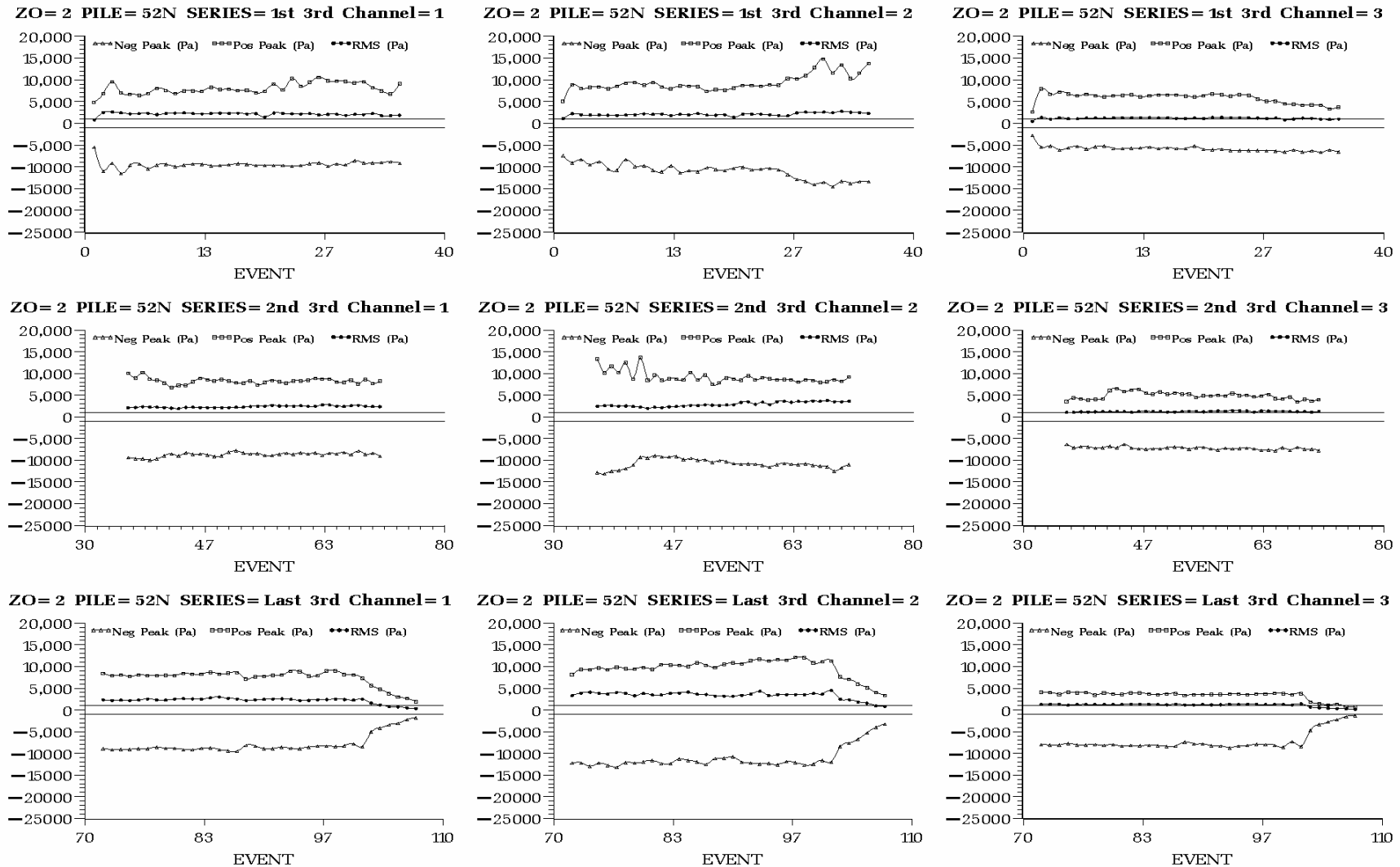
Figure C.2. Peak Positive, Peak Negative, and Root Mean Square Sound Pressure (Pa) of Each Impact at Plumb Pile 52N Driven in 40 ft Water with Type II Confined Bubble Curtain in Place. Plots are arranged by hydrophone H1 (left) to H3 (right) and by impact series, each containing one third of the impacts, from first third (top) to last third (bottom).
