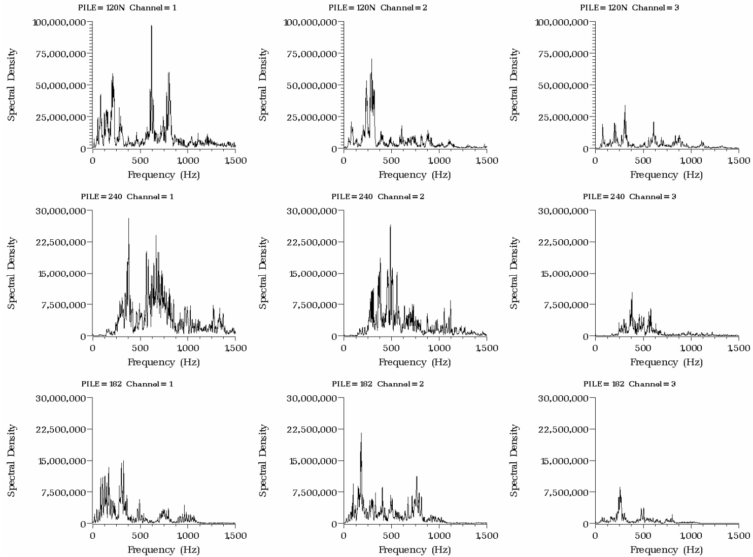
Figure E.5. Spectral Density (Pa 2 /Hz) versus Frequency (Hz) at Hydrophones H1 (left), H2 (center), and H3 (right) for the First 20 Impacts on Piles 120N, 240 (plumb piles driven without bubble curtain in place), and 182 (batter pile driven with Type I unconfined bubble curtain)
