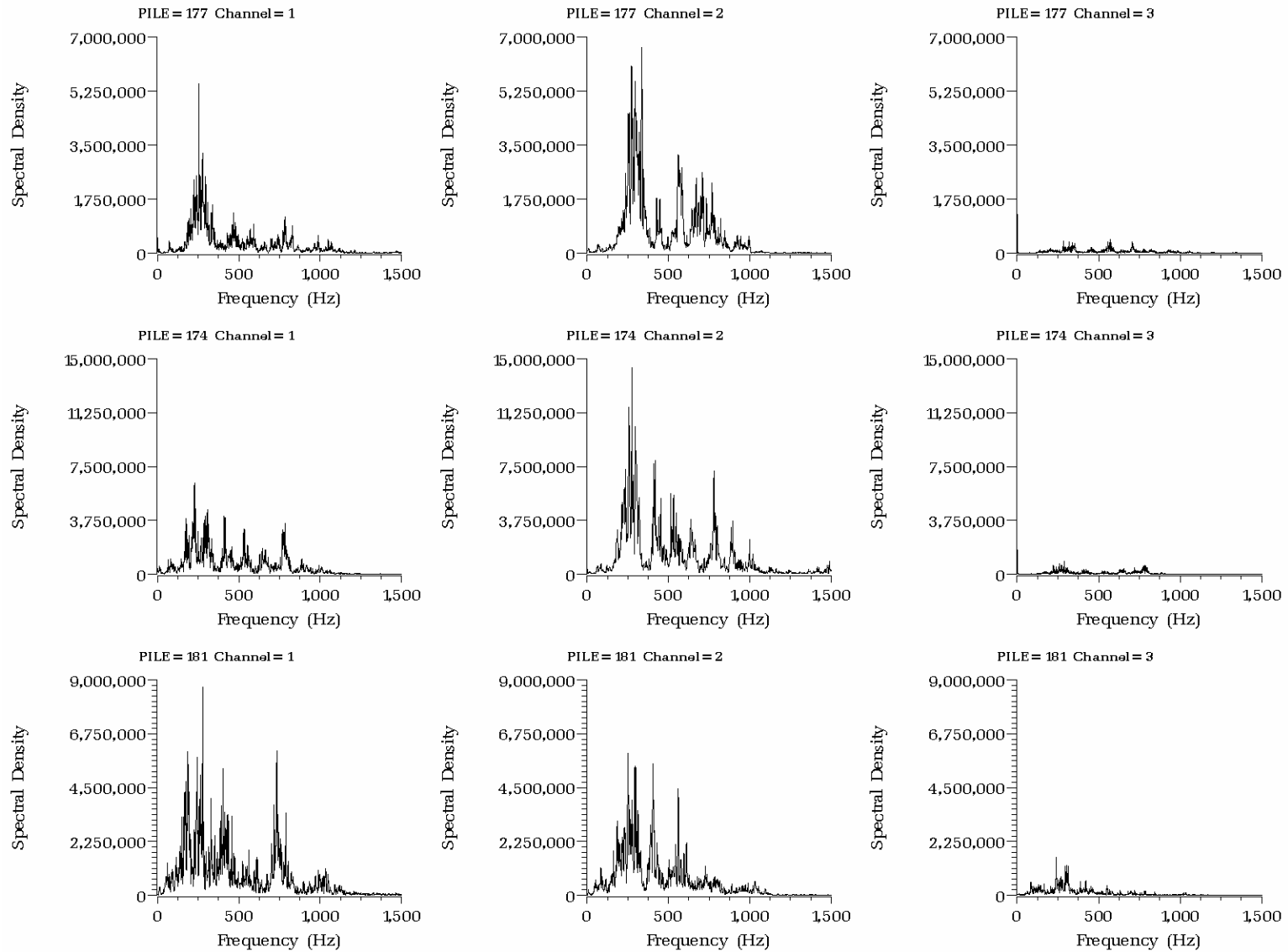
Figure E.6. Spectral Density (Pa 2 /Hz) versus Frequency (Hz) at Hydrophones H1 (left), H2 (center), and H3 (right) for the First 20 Impacts on Piles 177, 174, and 181 (all batter piles driven with Type I unconfined bubble curtain in place)
