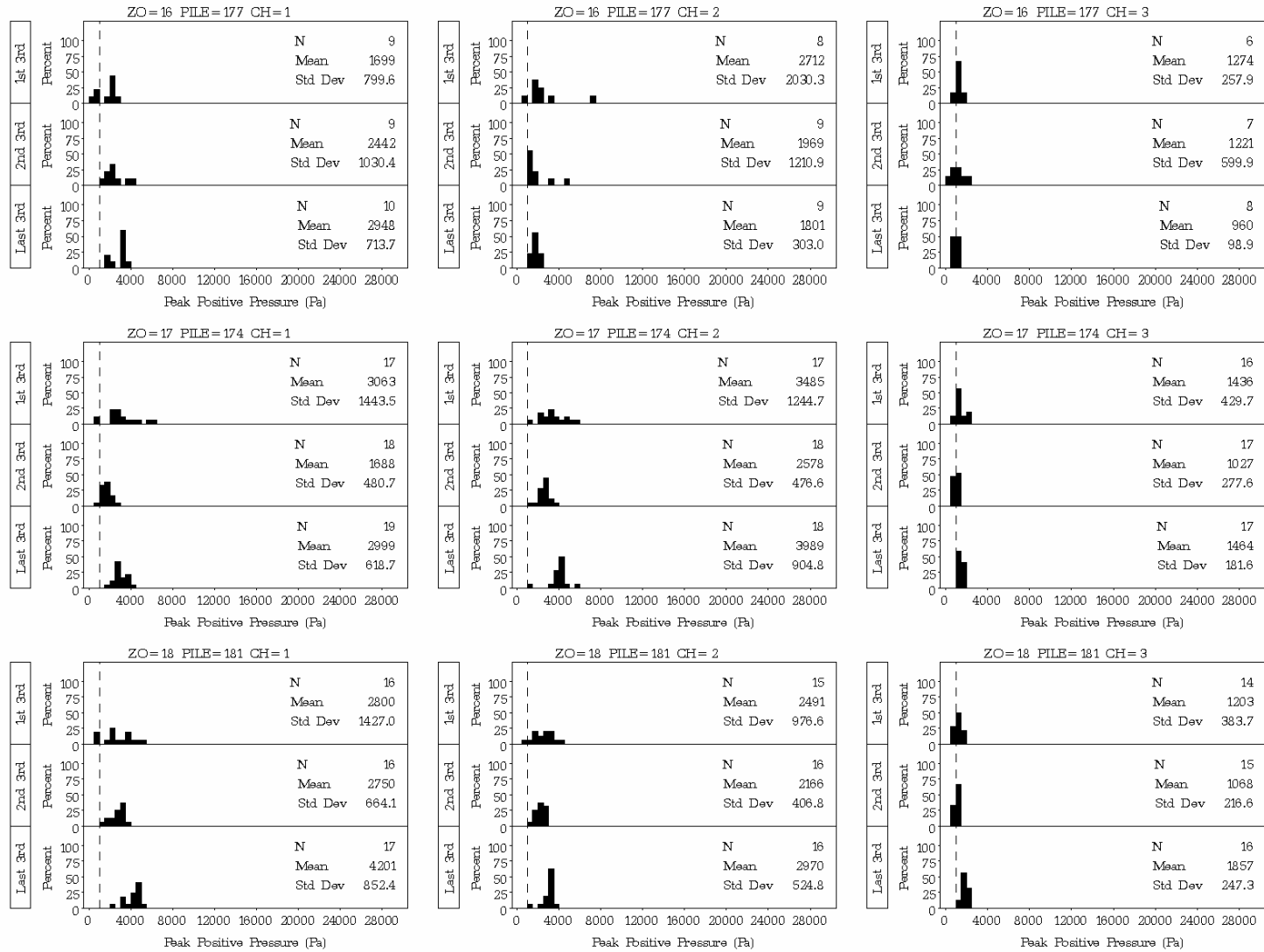
Figure D.13. Plots of Distribution Statistics on Peak Positive Pressure for Impacts on Batter Piles 177, 174, and 181 at the Hood Canal Bridge in 37 ft, 29 ft, and 33 ft of Water, Respectively, with Type I Unconfined Bubble Curtain in Place
