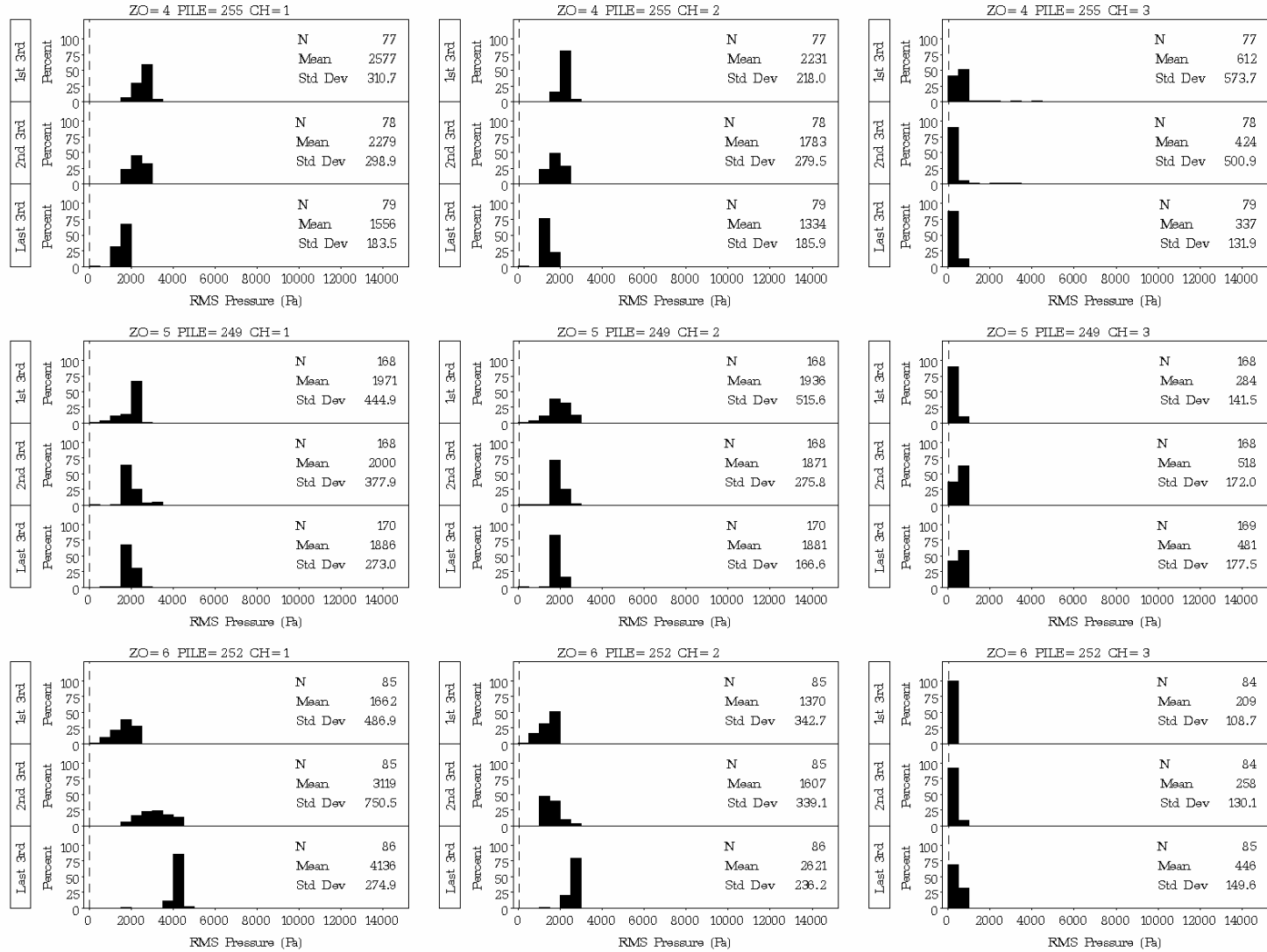
Figure D.2. Plots of Distribution Statistics on Root Mean Square Pressure for Impacts on Plumb Piles 255, 249, and 252 at the Hood Canal Bridge in 33 ft, 32 ft, and 31 ft of Water, Respectively, with Type II Confined Bubble Curtain in Place
