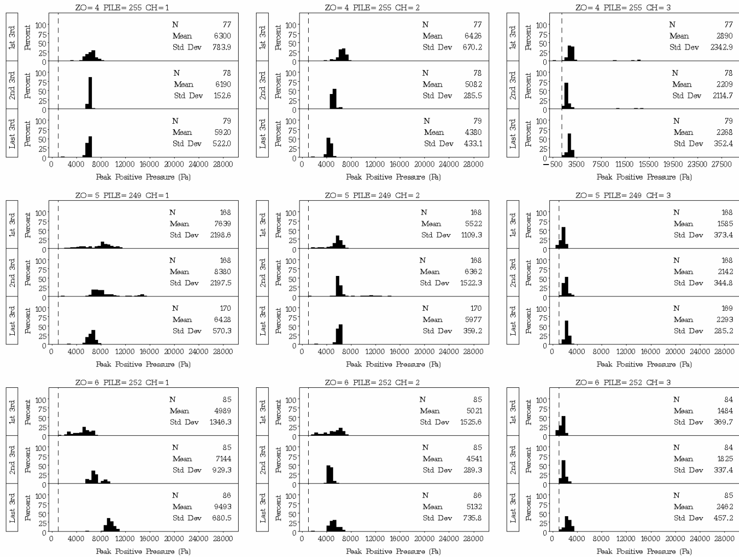
Figure D.9. Plots of Distribution Statistics on Peak Positive Pressure for Impacts on Plumb Piles 255, 249, and 252 at the Hood Canal Bridge in 33 ft, 32, ft, and 31 ft of Water, Respectively, with Type II Confined Bubble Curtain in Place
