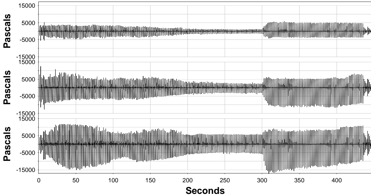
Figure A.1. Sound-Pressure Levels Measured by Hydrophones H1 (bottom), H2 (middle), and H3 (top) at Plumb Pile 121N Driven in 42 ft of Water with Bubble Curtain in Place
