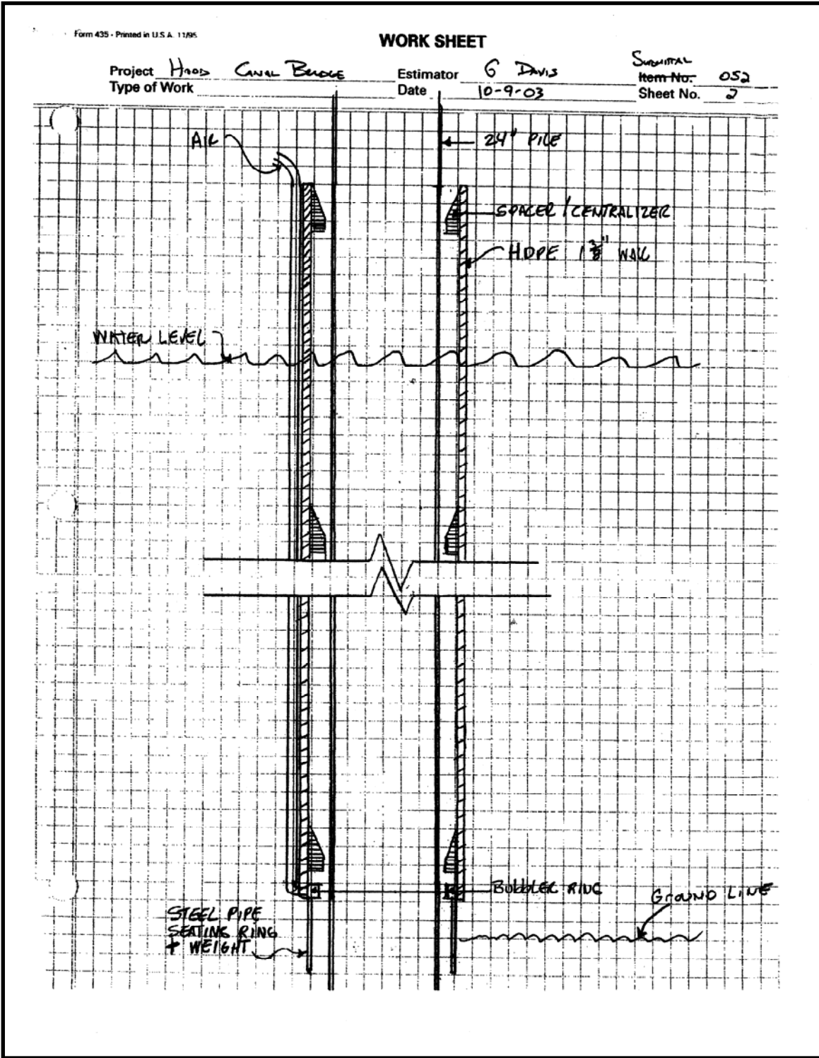
Figure F.3. Contractor's Side View Drawing of Bubble Ring for Confined Bubble Curtain used on Plumb Piles
