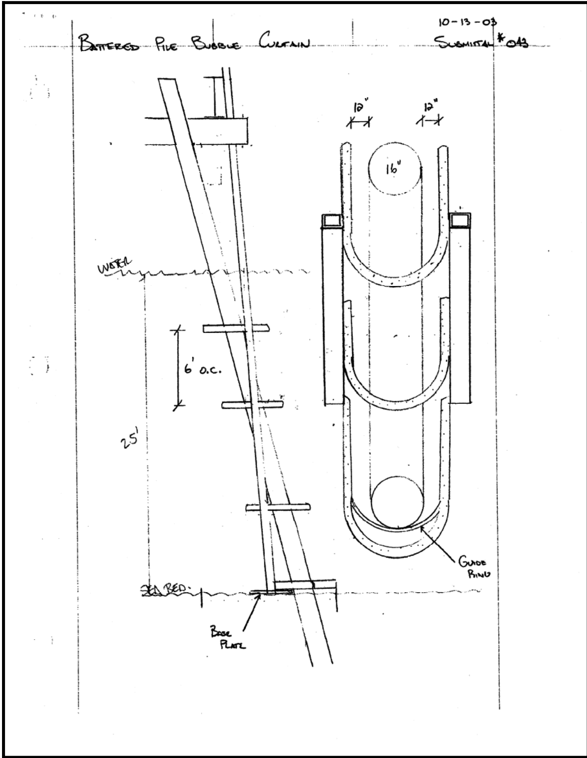
Figure F.7. Contractor's Side and Top View Drawings of Multiple Bubbler Unconfined Bubble Curtain Used on Battered Piles
