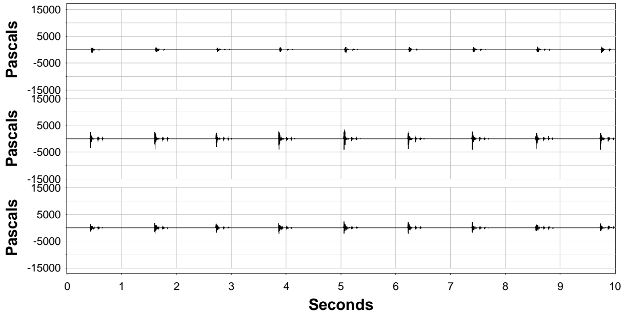
Figure 12. Sound-Pressure Levels Measured over Successive Impacts of Batter Pile 178 Driven in 37 ft of Water Without Bubble Curtain in Place (bottom, H1; middle, H2; top, H3)
