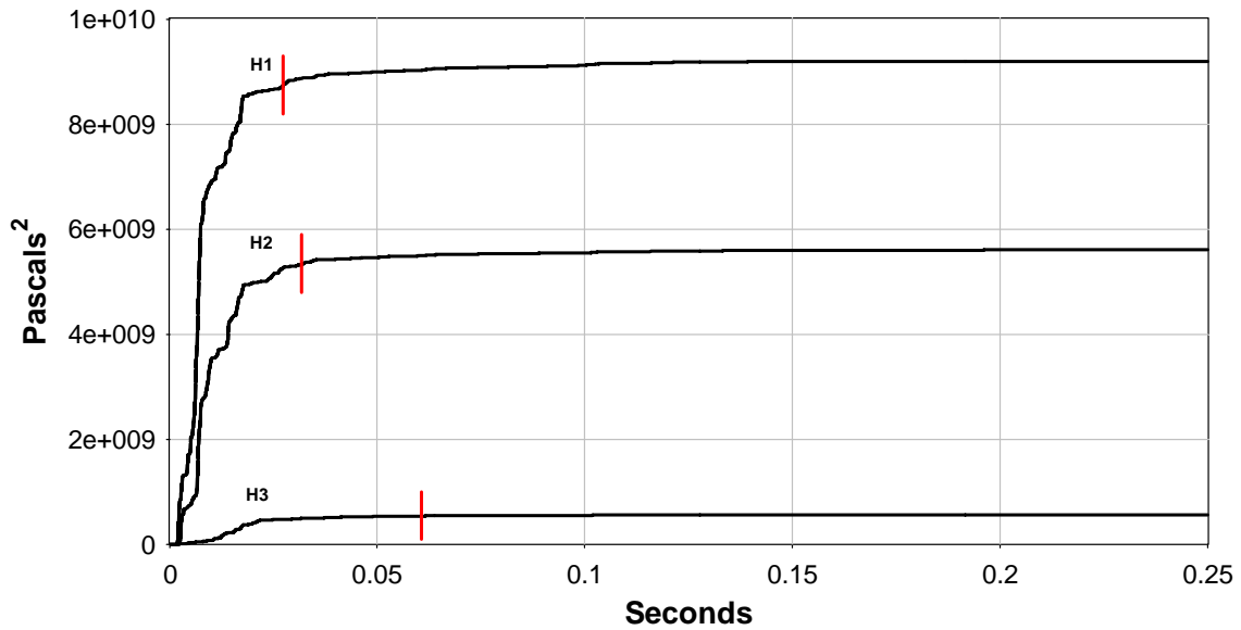
Figure 16. Power Spectral Density Indices (Figure 16a: H1 top plot, H2 middle plot, H3 bottom plot) and Cumulative Sound Exposure Over Time (Figure 16b) for a Single Pile-Driving Impact Measured at Plumb Pile 255, Driven in 33 ft of Water with Bubble Curtain. On the cumulative sound plot, the vertical lines represent the point in time when the summed squared sound pressures of the waveform total 95% of the sound energy.
