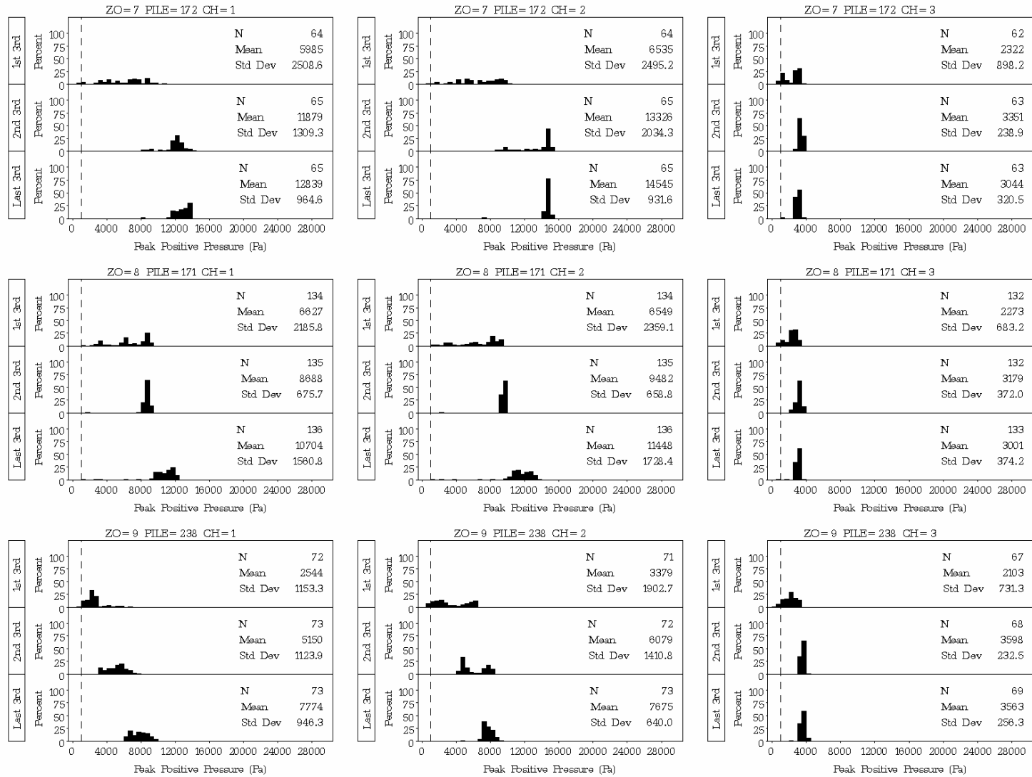
Figure D.10. Plots of Distribution Statistics on Peak Positive Pressure for Impacts on Plumb Piles 172, 171, and 238 at the Hood Canal Bridge in 20 ft, 18 ft, and 7 ft of Water, Respectively, with Type II Confined Bubble Curtain in Place
