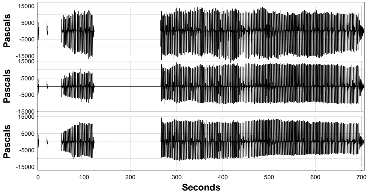
Figure A.12. Sound-Pressure Levels (Pa) Measured for Plumb Pile 50N Driven in 40 ft of Water with No Bubble Curtain.
