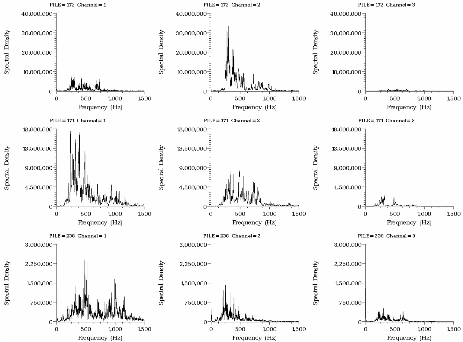
Figure E.3. Spectral Density (Pa 2 /Hz) Versus Frequency (Hz) at Hydrophones H1 (left), H2 (center), and H3 (right) for the First 20 Impacts on Piles 172, 171, and 238 (all plumb piles driven with Type II confined bubble curtain in place)
