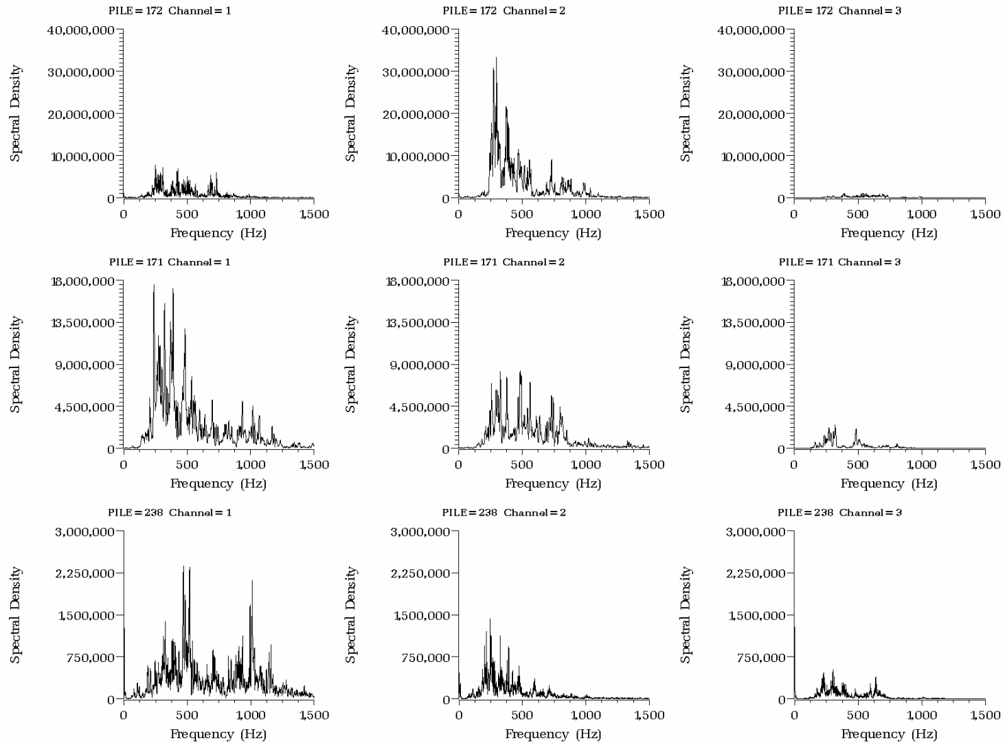
Figure 15. Example of Plots of Spectral Density Indices (Pa 2 /Hz) versus Frequency (Hz) at Each Hydrophone (H1, H2, H3 from left to right) for First 20 Impacts on Plumb Piles 172, 171, and 238
