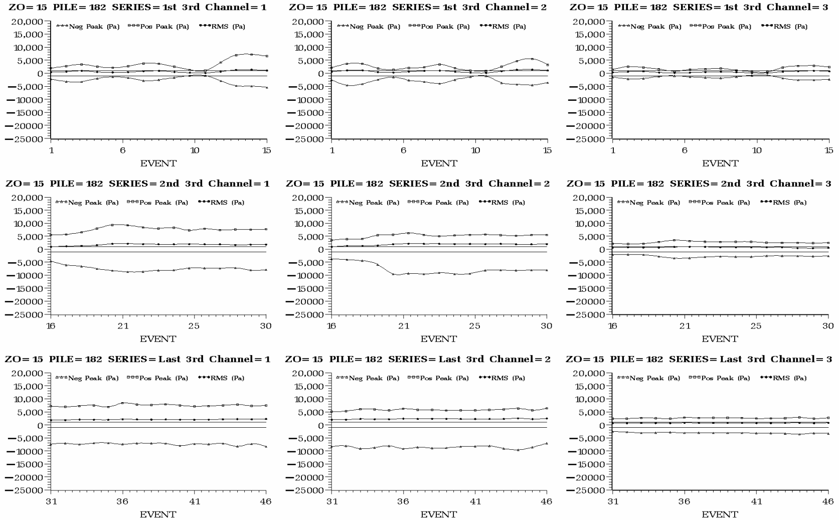
Figure C.15. Peak Positive, Peak Negative, and Root Mean Square Sound Pressure (Pa) of Each Impact on Batter Pile 182 Driven at Hood Canal Bridge in 41 ft of Water with a Type I Unconfined Bubble Curtain in Place. Plots are arranged by hydrophone H1 (left) to H3 (right) and by impact series, each containing one third of the impacts, from first third (top) to last third (bottom).
