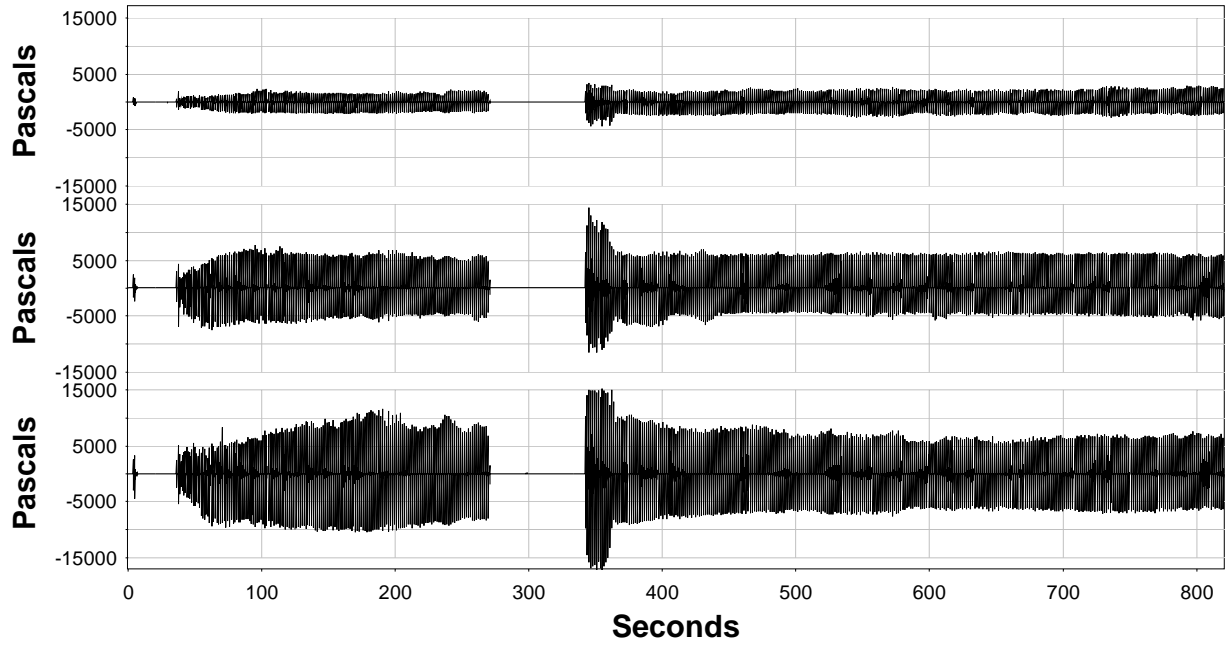
Figure A.5. Sound-Pressure Levels (Pa) Measured for Plumb Pile 249 Driven in 32 ft of Water with the Bubble Curtain in Place.
