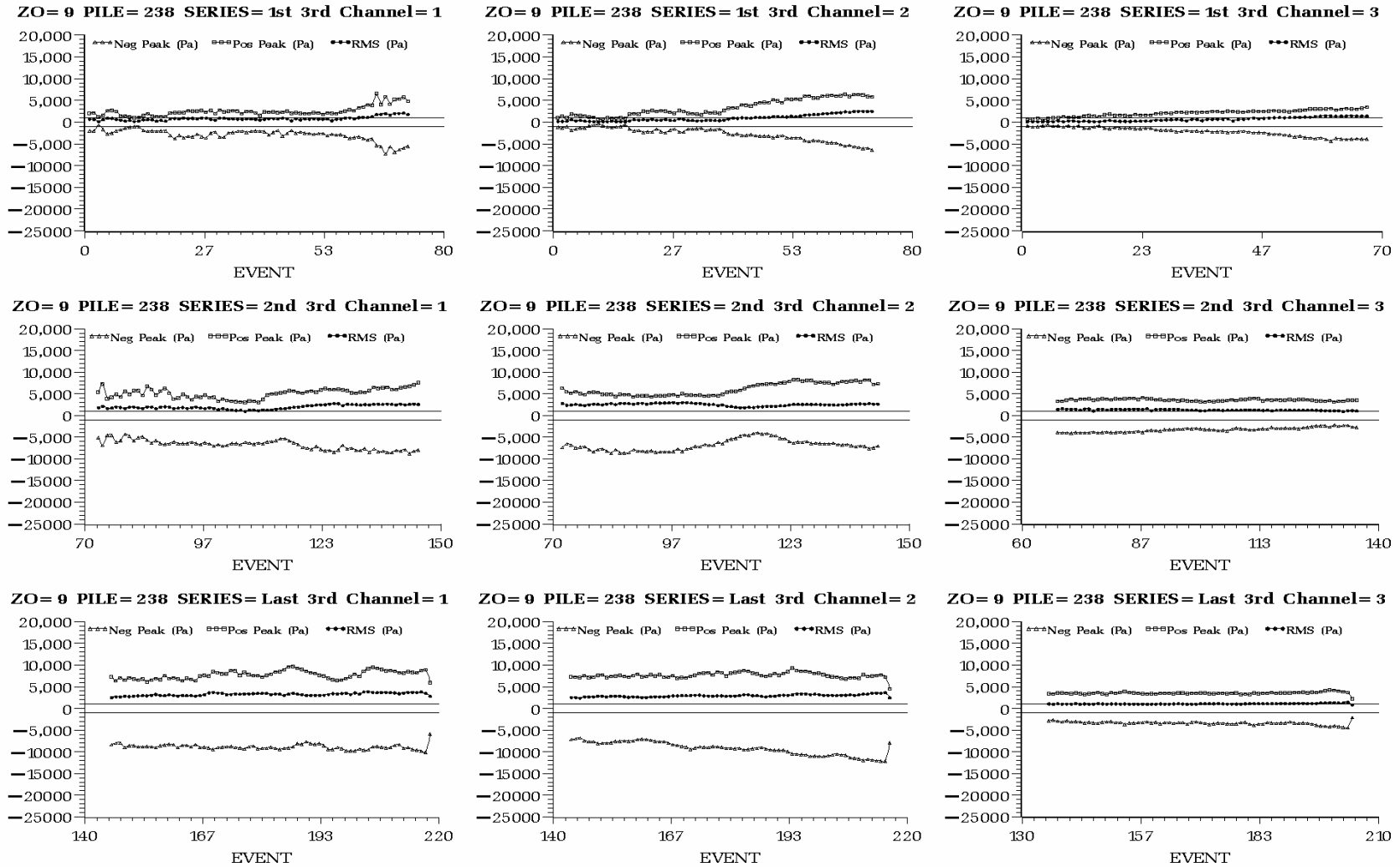
Figure C.9. Peak Positive, Peak Negative, and Root Mean Square Sound Pressure (Pa) of Each Impact on Plumb Pile 238 Driven at Hood Canal Bridge in 7 ft of Water with a Type II Confined Bubble Curtain in Place. Plots are arranged by hydrophone H1 (left) to H3 (right) and by impact series, each containing one third of the impacts, from first third (top) to last third (bottom).
