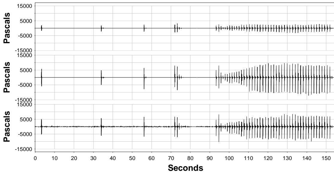
Figure 14. Sound-Pressure Levels (Pa) measured for batter pile 178 driven in 37 ft of water with no bubble curtain. H1 (bottom plot), H2 (middle plot), and H3 (top plot).
