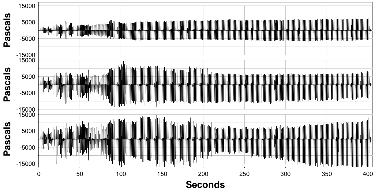
Figure A.14. Sound-Pressure Levels (Pa) Measured for Plumb Pile 240 Driven in 9 ft of Water with No Bubble Curtain.
