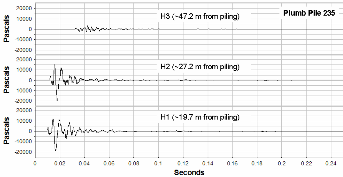
Figure 9. Sound-Pressure Levels Measured for a Single Impact of Plumb Pile 235 Driven in 4.5 ft of Water with the Bubble Curtain in Place (bottom, H1; middle, H2; top, H3)
