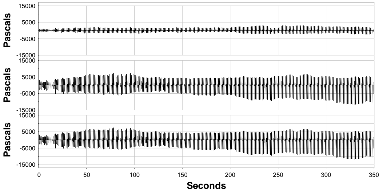
Figure A.6. Sound-Pressure Levels (Pa) Measured for Plumb Pile 252 Driven in 31 ft of Water with the Bubble Curtain in Place.
