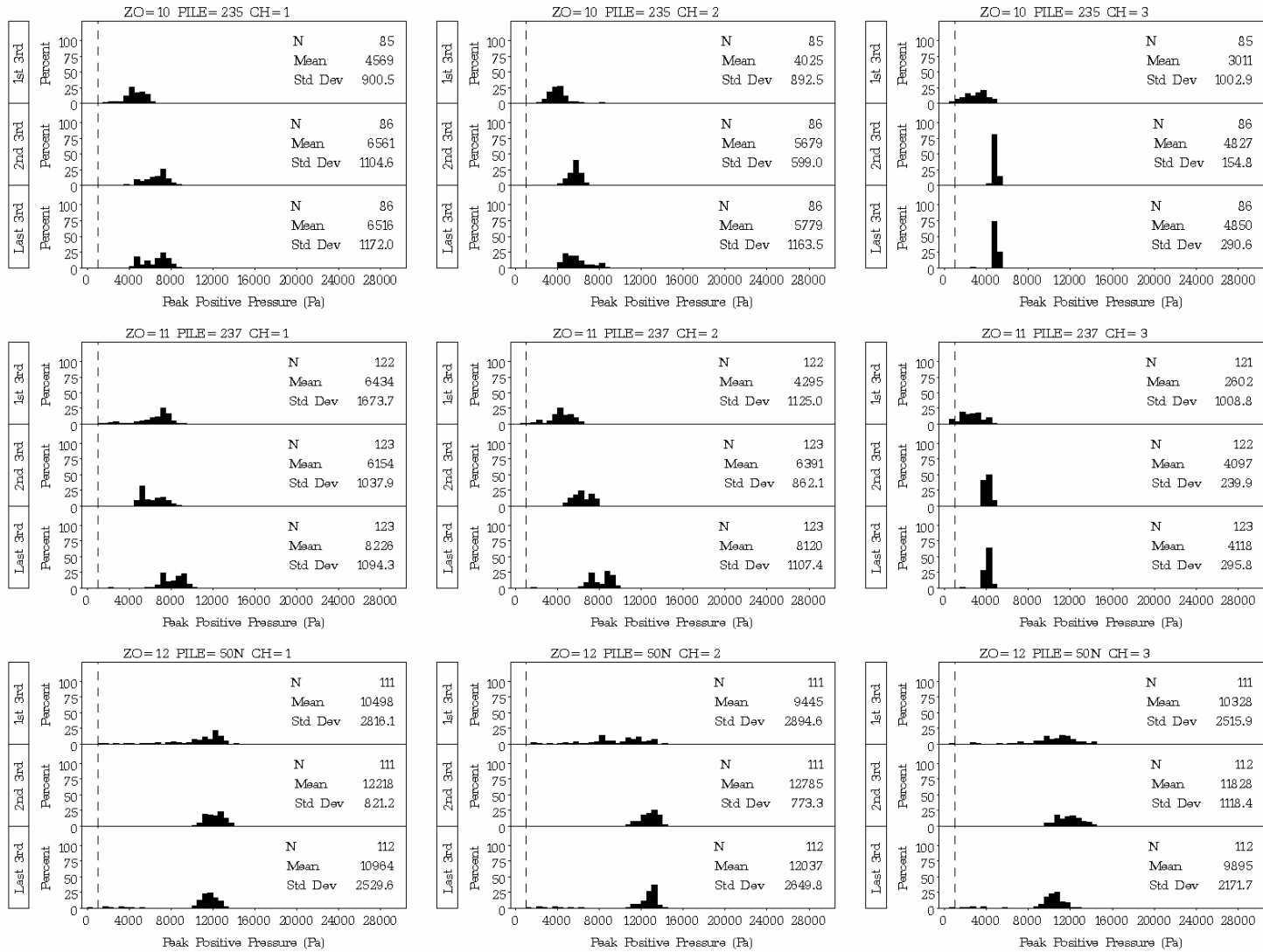
Figure D.11. Plots of Distribution Statistics on Peak Positive Pressure for Impacts on Plumb Piles 235 and 237 in 4.5 ft and 4 ft of Water, Respectively, with a Type II Confined Bubble Curtain in Place, and at Plumb Pile 50N in 40 ft of Water with No Bubble Curtain in Place
