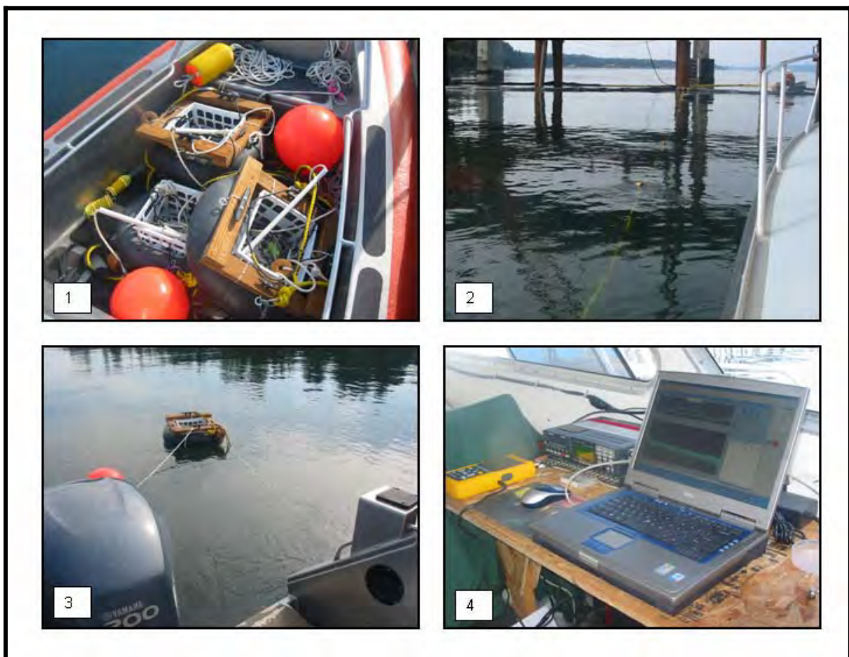
Figure 7. Hydrophone Array Deployment: 1) hydrophones and floats in vessel ready to deploy along floating backbone line; 2) floating backbone line extending parallel to shore from piling; 3) deployed hydrophone float connected to data acquisition system; and 4) shipboard data acquisition system
