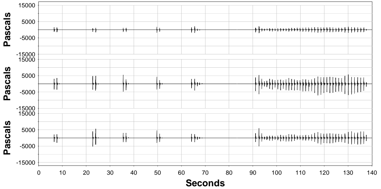
Figure A.17. Sound-Pressure Levels (Pa) Measured for Batter Pile 174 Driven in 29 ft of Water with the Bubble Curtain in Place.
