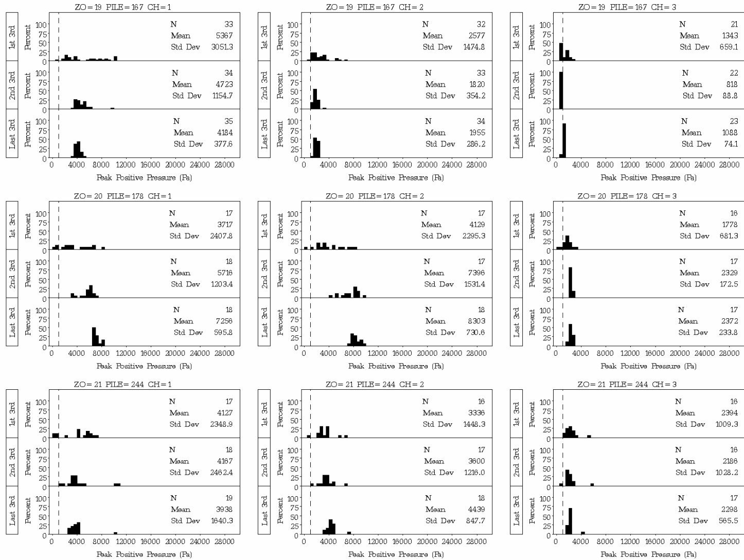
Figure D.14. Plots of Distribution Statistics on Peak Positive Pressure for Impacts on Piles Batter Piles 167, 178, and 244 at the Hood Canal Bridge. Batter pile 167 is in 7 ft of water with a Type I unconfined bubble curtain in place; batter piles 178 and 244 are in 37 ft and 20 ft of water, respectively, with no bubble curtains in place.
