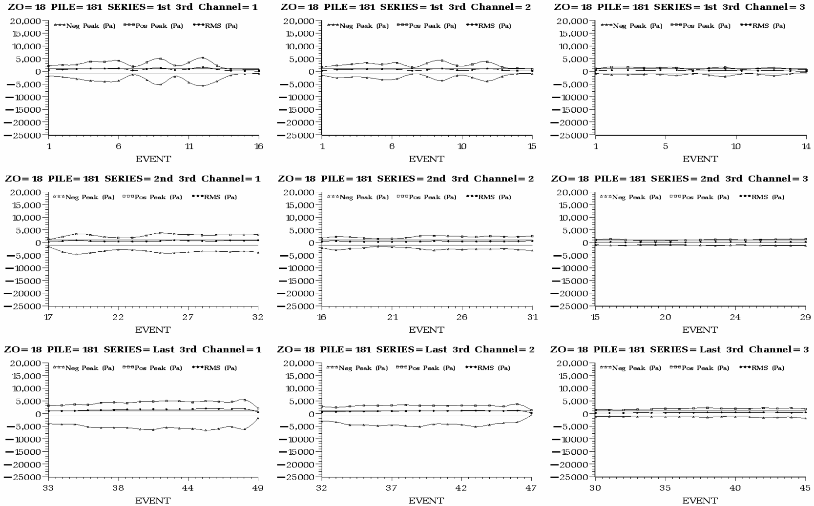
Figure C.18. Peak Positive, Peak Negative, and Root Mean Square Sound Pressure (Pa) of Each Impact on Batter Pile 181 Driven at Hood Canal Bridge in 33 ft of Water with a Type I Unconfined Bubble Curtain in Place. Plots are arranged by hydrophone H1 (left) to H3 (right) and by impact series, each containing one third of the impacts, from first third (top) to last third (bottom).
