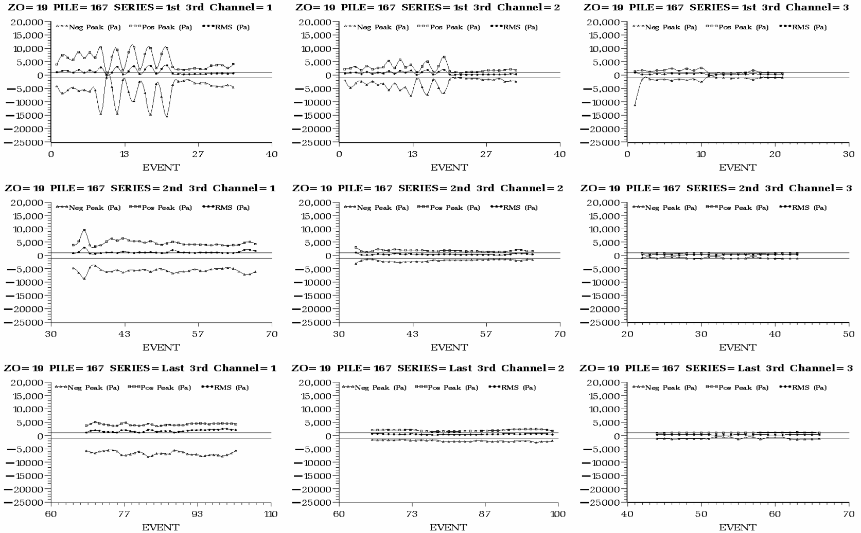
Figure C.19, Peak Positive, Peak Negative, and Root Mean Square Sound Pressure (Pa) of Each Impact on Batter Pile 167 Driven at Hood Canal Bridge in 7 ft of Water with a Type I Unconfined Bubble Curtain in Place. Plots are arranged by hydrophone H1 (left) to H3 (right) and by impact series, each containing one third of the impacts, from first third (top) to last third (bottom).
