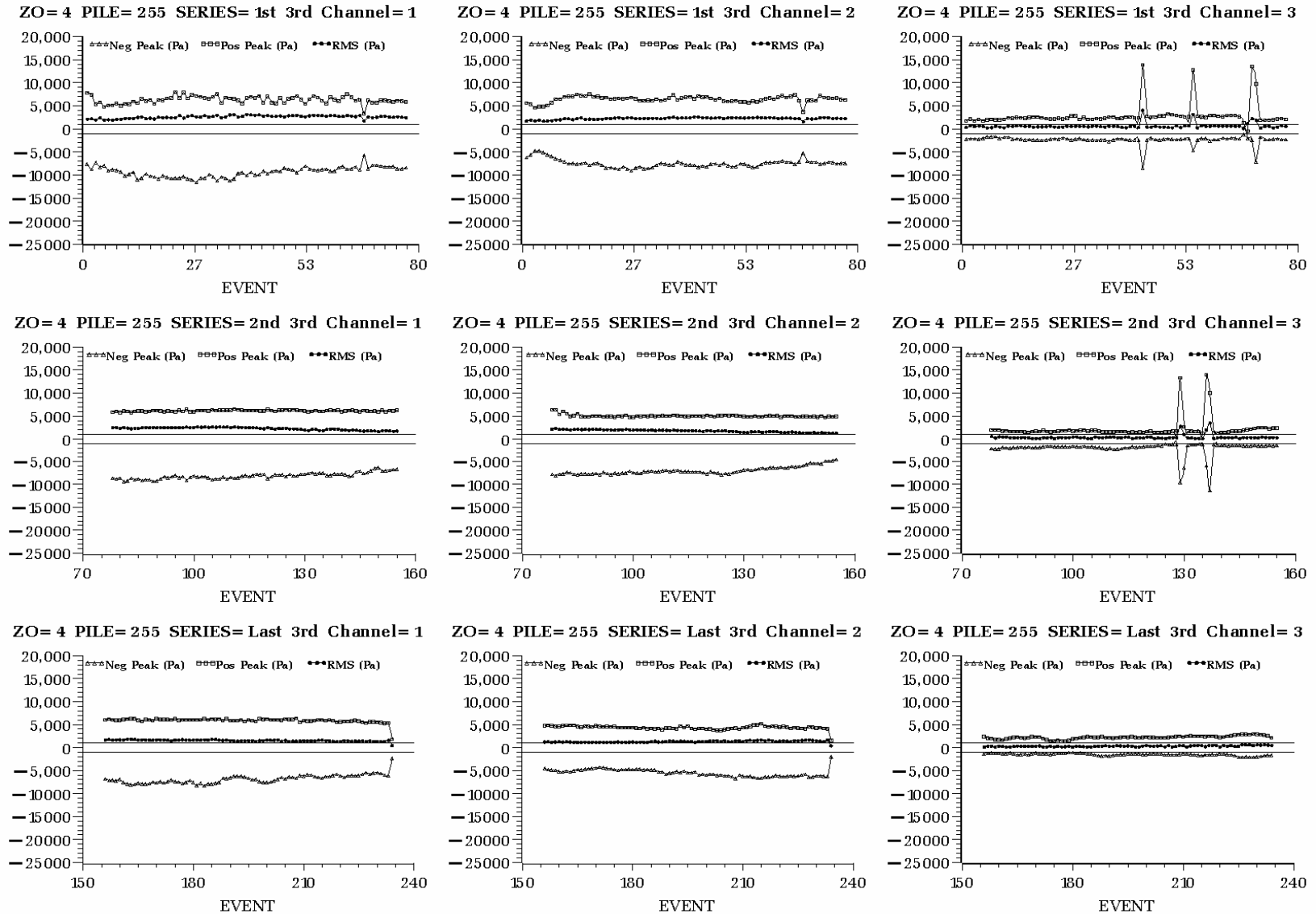
Figure C.4. Peak Positive, Peak Negative, and Root Mean Square Sound Pressure (Pa) of Each Impact at Plumb Pile 255 Driven in 33 ft of Water with Type II Confined Bubble Curtain in Place. Plots are arranged by hydrophone H1 (left) to H3 (right) and by impact series, each containing one third of the impacts, from first third (top) to last third (bottom).
