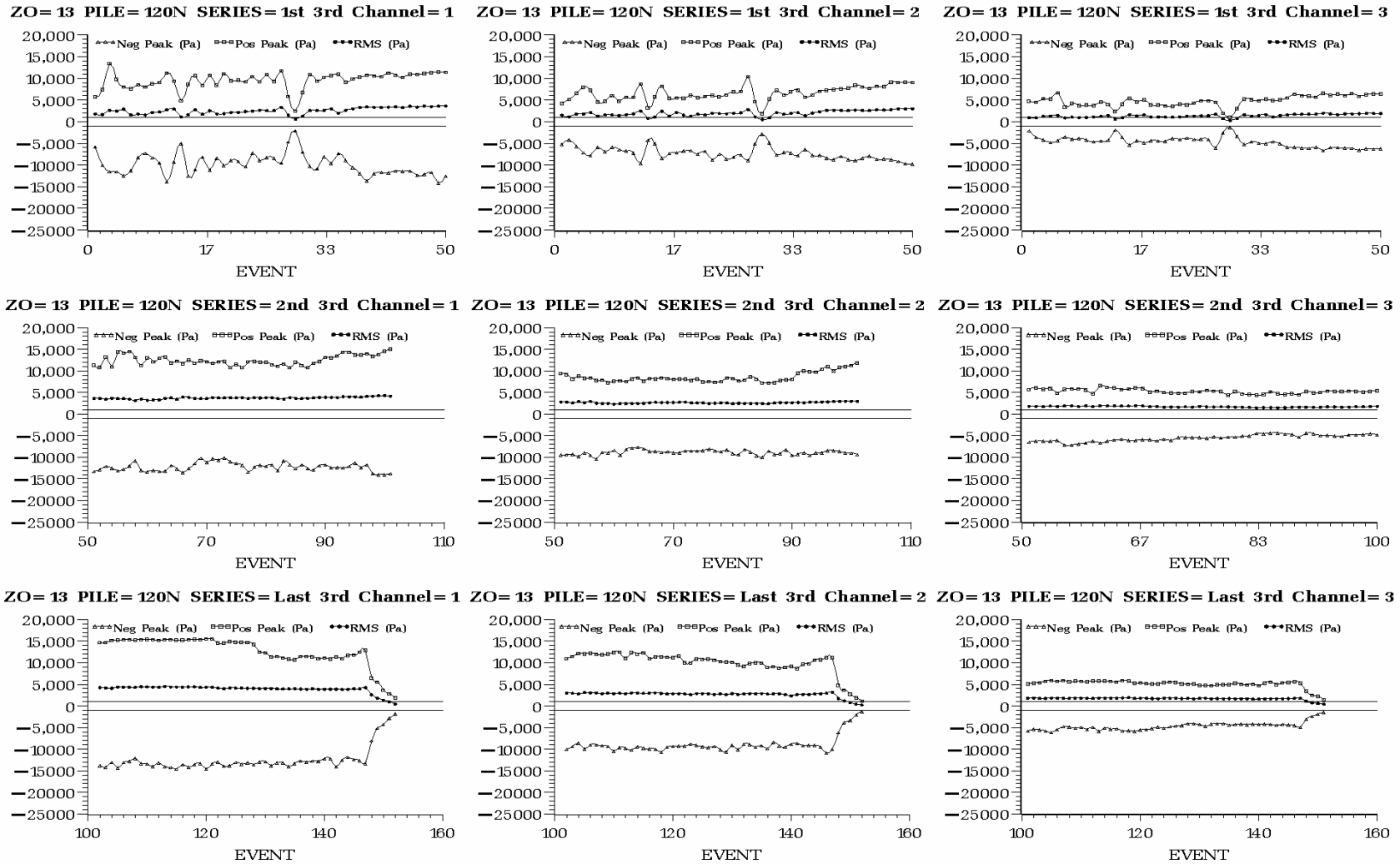
Figure C.13. Peak Positive, Peak Negative, and Root Mean Square Sound Pressure (Pa) of Each Impact on Plumb Pile 120N Driven at Hood Canal Bridge in 39 ft of Water with No Bubble Curtain in Place. Plots are arranged by hydrophone H1 (left) to H3 (right) and by impact series, each containing one third of the impacts, from first third (top) to last third (bottom).
