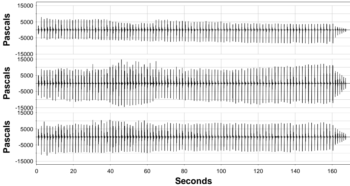
Figure A.2. Sound-Pressure Levels Measured by Hydrophones H1 (bottom), H2 (middle), and H3 (top) at Plumb Pile 52N Driven in 40 ft of Water with Bubble Curtain in Place
