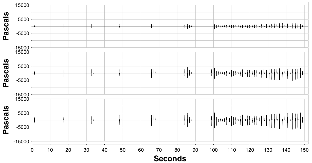
Figure A.18. Sound-Pressure Levels (Pa) Measured for Batter Pile 181 Driven in 7 ft of Water with the Bubble Curtain in Place.
