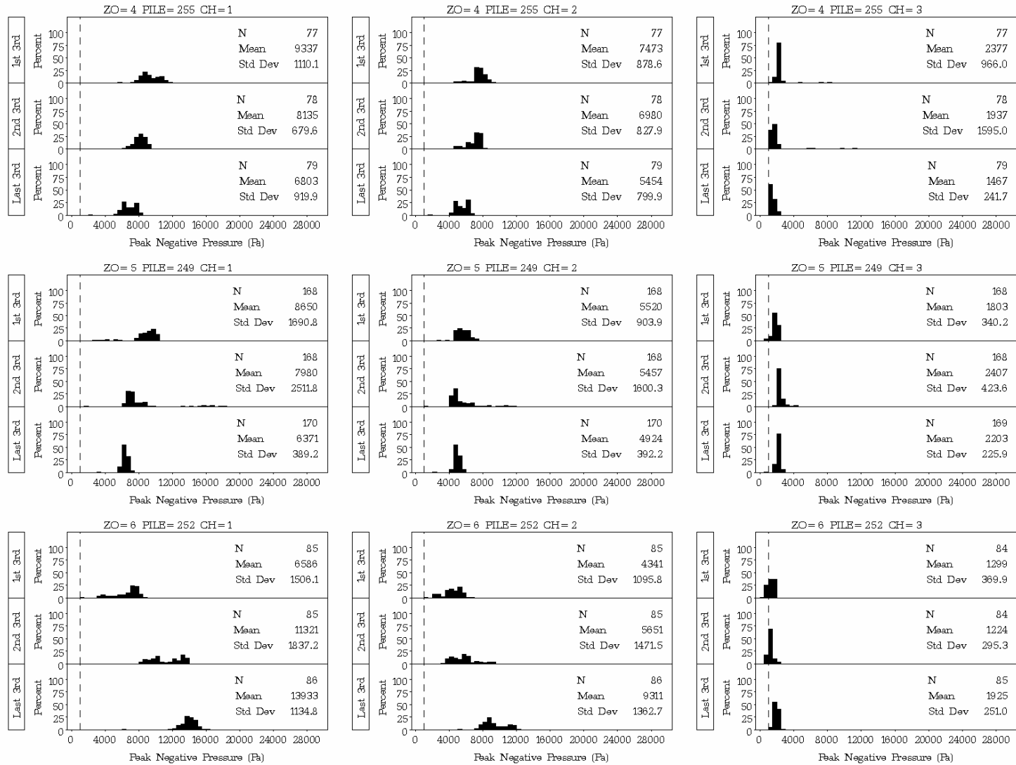
Figure D.16. Plots of Distribution Statistics on Peak Negative Pressure for Impacts on Plumb Piles 255, 249, and 252 at the Hood Canal Bridge in 33 ft, 32 ft, and 31 ft of Water, Respectively, with Type II Confined Bubble Curtain in Place
