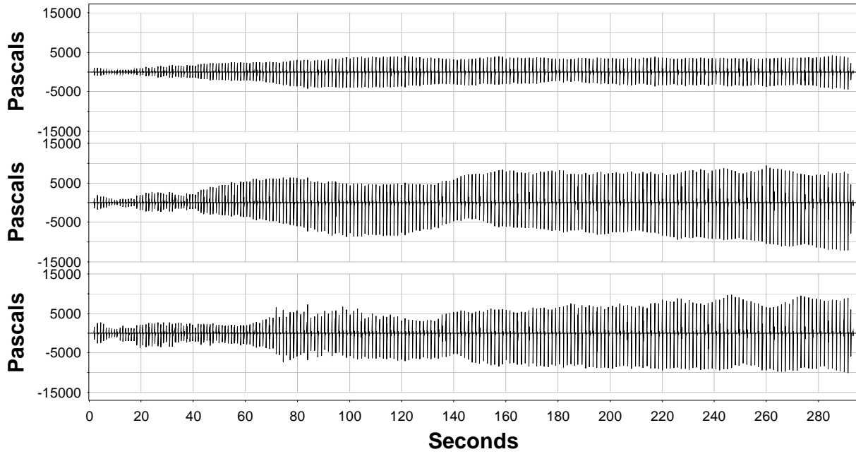
Figure A.9. Sound-Pressure Levels (Pa) Measured for Plumb Pile 238 Driven in 7 ft of Water with the Bubble Curtain in Place.
