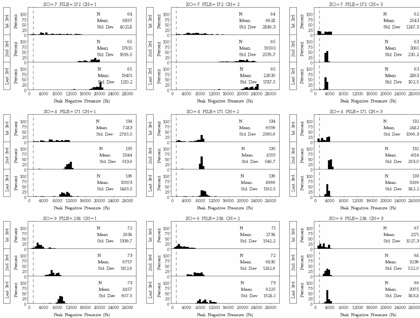
Figure D.17. Plots of Distribution Statistics on Peak Negative Pressure for Impacts on Plumb Piles 172, 171, and 238 at the Hood Canal Bridge in 20 ft, 18 ft, and 7 ft of Water, Respectively, with a Type II Confined Bubble Curtain in Place
