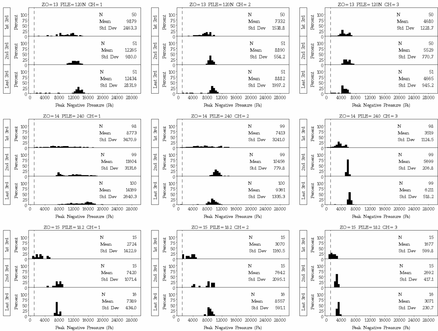
Figure D.19. Plots of Distribution Statistics on Peak Negative Pressure for Impacts on Plumb Piles 120N and 240 in 39 ft and 9 ft of Water, Respectively, with No Bubble Curtain in Place, and on Batter Pile 182 in 41 ft of Water with No Bubble Curtain in Place
