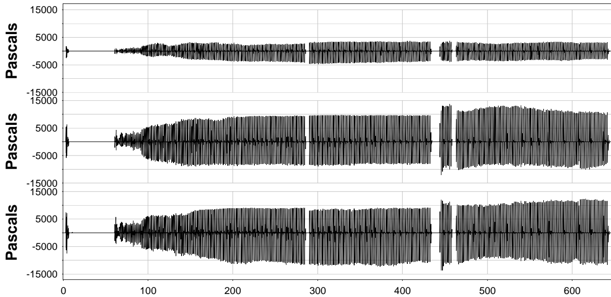
Figure A.8. Sound-Pressure Levels (Pa) Measured for Plumb Pile 171 Driven in 18 ft of Water with the Bubble Curtain in Place.
