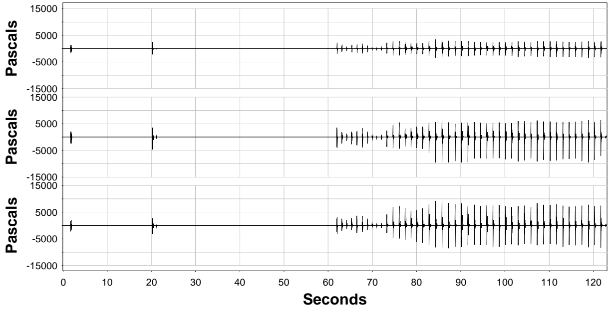
Figure A.15. Sound-Pressure Levels (Pa) Measured for Batter Pile 182 Driven in 41 ft of Water with the Bubble Curtain in Place.
