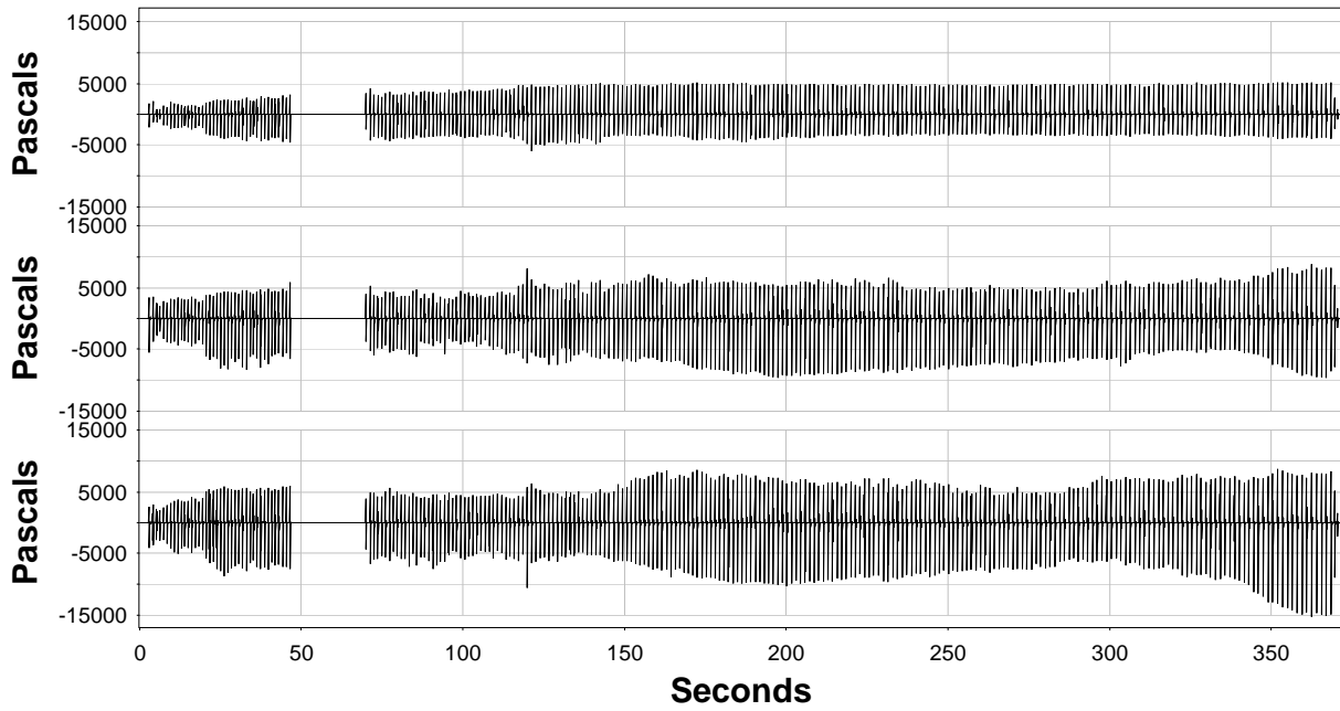
Figure A.10. Sound-Pressure Levels (Pa) Measured for Plumb Pile 235 Driven in 4.5 ft of Water with the Bubble Curtain in Place.
