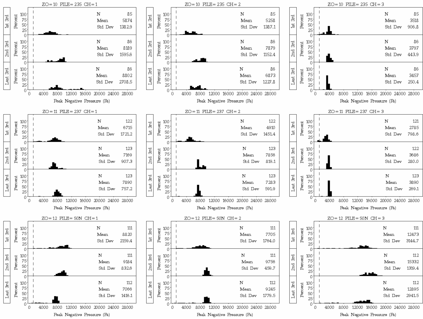
Figure D.18. Plots of Distribution Statistics on Peak Negative Pressure for Impacts on Plumb Piles 235 and 237 in 4.5 ft and 4 ft of Water, Respectively, with a Type II Confined Bubble Curtain in Place, and at Plumb Pile 50N in 40 ft of Water with No Bubble Curtain in Place
