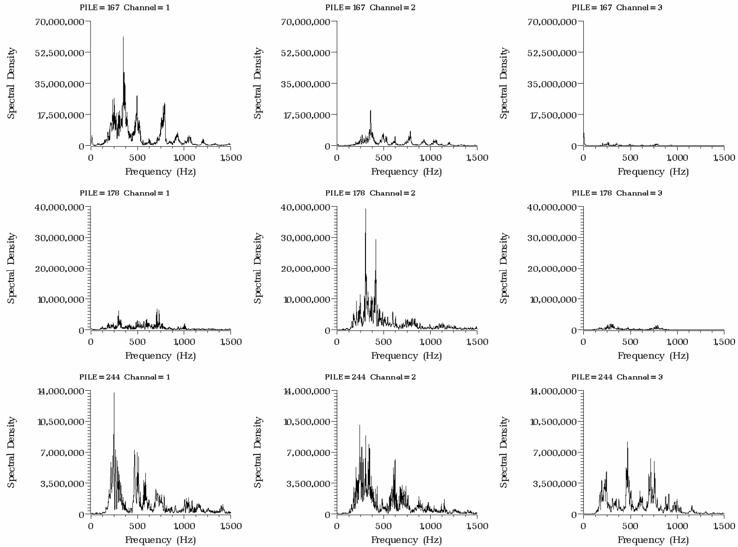
Figure E.7. Spectral Density (Pa 2 /Hz) versus Frequency (Hz) at Hydrophones H1 (left), H2 (center), and H3 (right) for the First 20 Impacts on Piles 167 (batter pile driven with Type I unconfined bubble curtain in place), and 178 and 244 (batter piles driven without bubble curtain)
