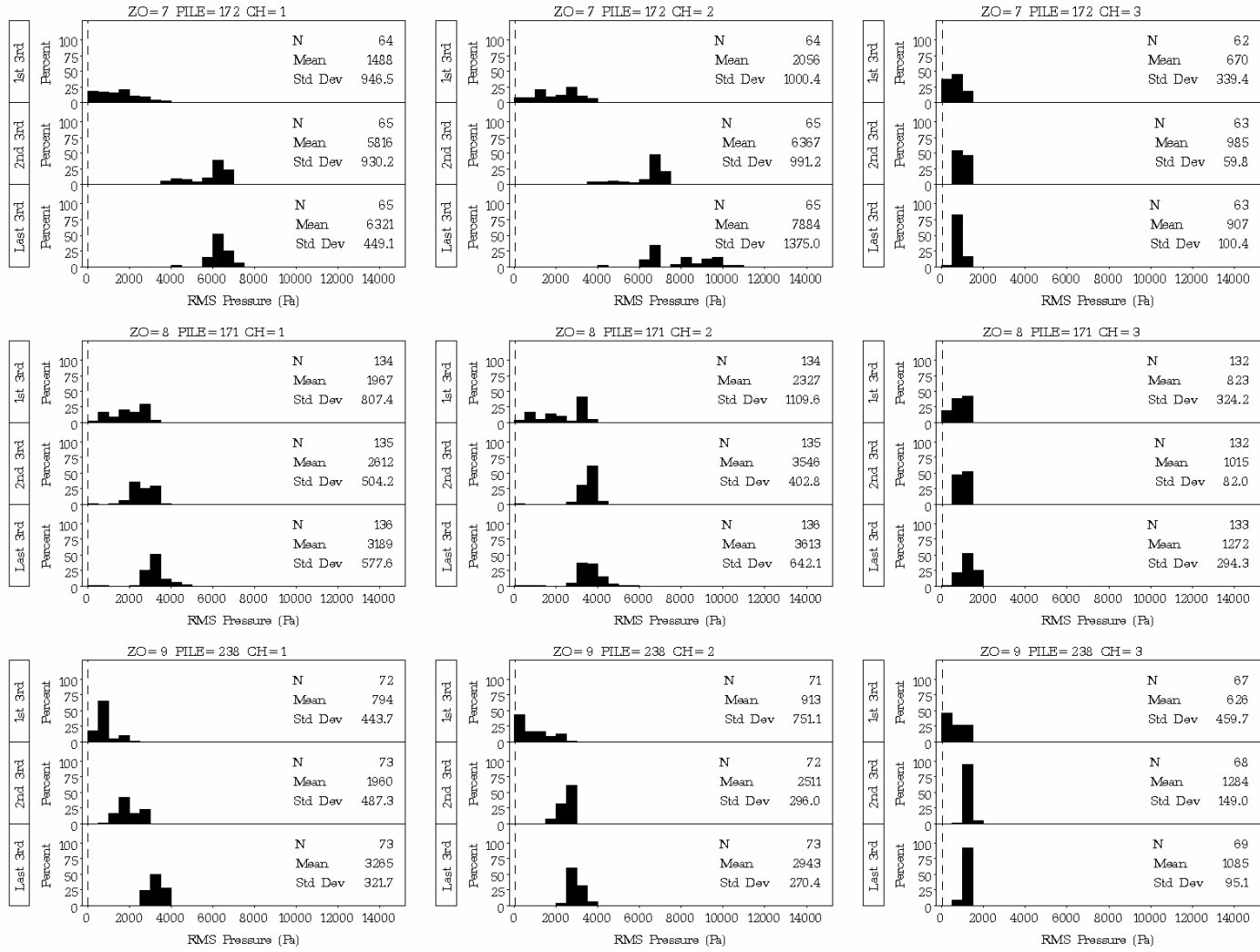
Figure D.3. Plots of Distribution Statistics on Root Mean Square Pressure for Impacts on Plumb Piles 172, 171, and 238 at the Hood Canal Bridge in 20 ft, 18 ft, and 7 ft of Water, Respectively, with Type II Confined Bubble Curtain in Place
