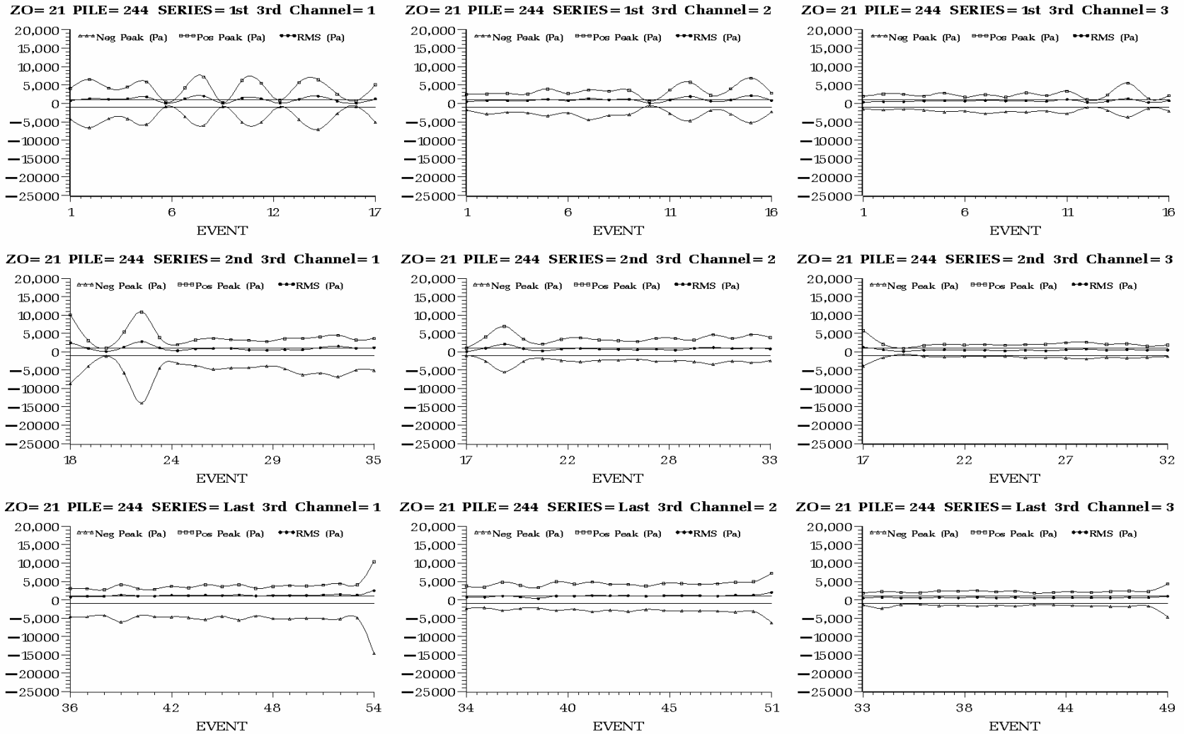
Figure C.21. Peak Positive, Peak Negative, and Root Mean Square Sound Pressure (Pa) of Each Impact on Batter Pile 244 Driven at Hood Canal Bridge in 20 ft of Water with No Bubble Curtain in Place. Plots are arranged by hydrophone H1 (left) to H3 (right) and by impact series, each containing one third of the impacts, from first third (top) to last third (bottom).
