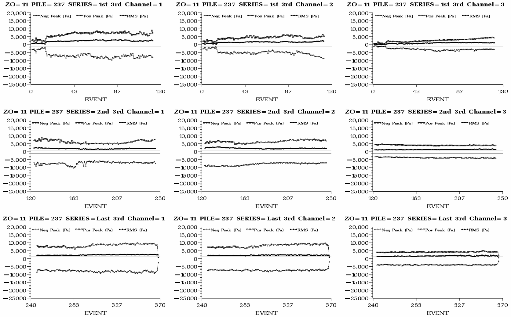
Figure C.11. Peak Positive, Peak Negative, and Root Mean Square Sound Pressure (Pa) of Each Impact on Plumb Pile 237 Driven at Hood Canal Bridge in 4 ft of Water with a Type II Confined Bubble Curtain in Place. Plots are arranged by hydrophone H1 (left) to H3 (right) and by impact series, each containing one third of the impacts, from first third (top) to last third (bottom).
