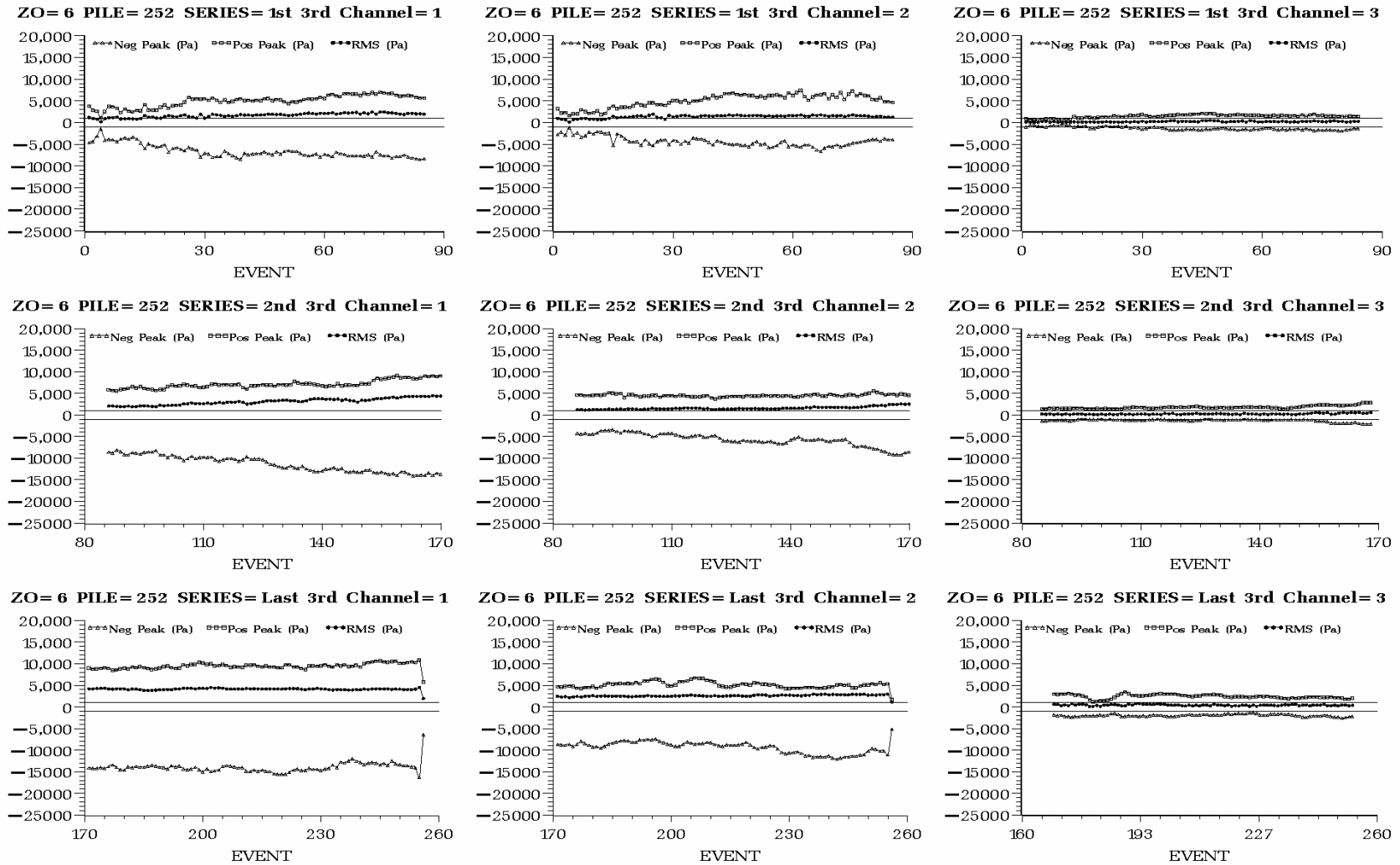
Figure C.6. Peak Positive, Peak Negative, and Root Mean Square Sound Pressure (Pa) of Each Impact on Plumb Pile 252 Driven at Hood Canal Bridge in 31 ft of Water with a Type II Confined Bubble Curtain in Place. Plots are arranged by hydrophone H1 (left) to H3 (right) and by impact series, each containing one third of the impacts, from first third (top) to last third (bottom).
