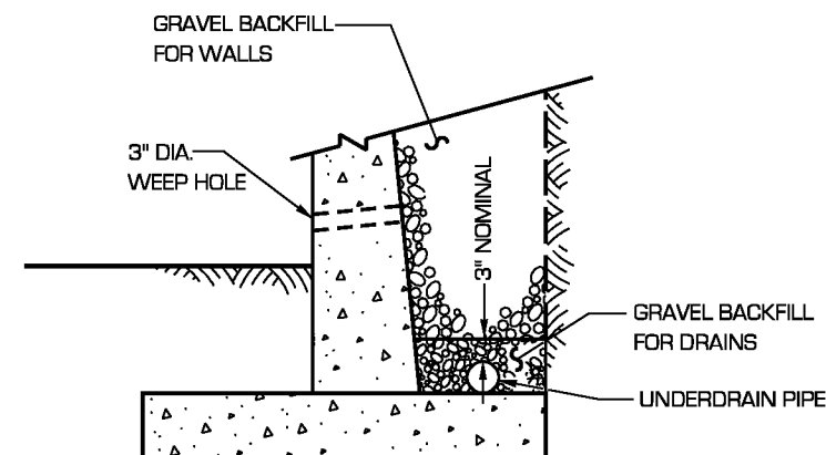
ALTERNATE DETAIL TYPICAL FOR CONSTRUCTION WITH SHORING.
