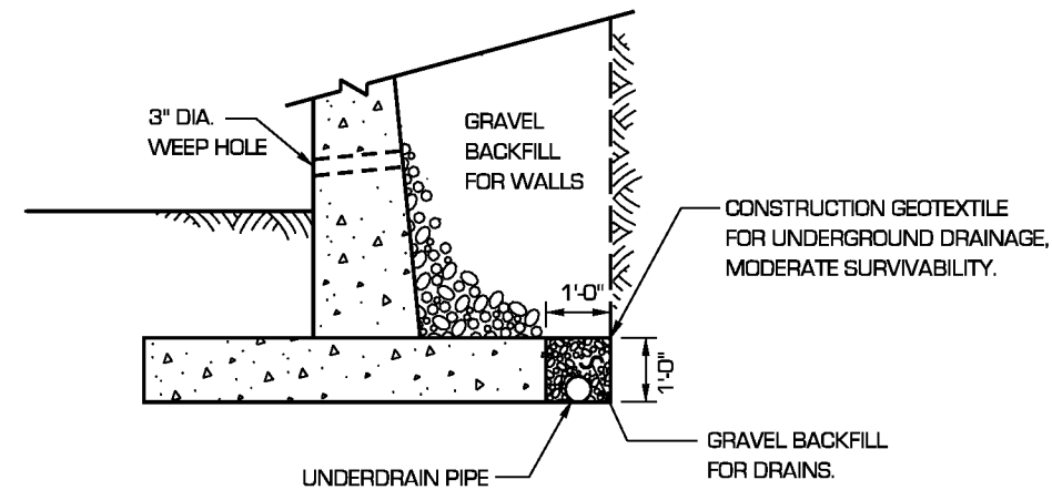
CONDITION A OR CONDITION B WITH GEOTEXTILE
