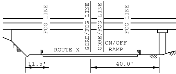
FREEWAY ON/OFF RAMP
