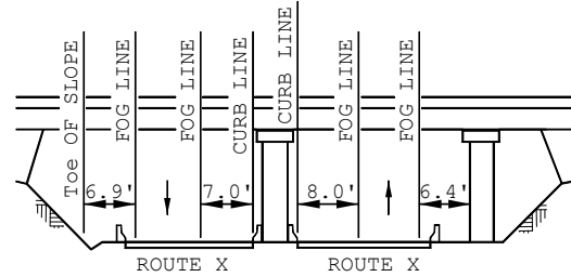
FREEWAY PIER MEDIAN WITH BARRIER ADJACENT TO SUBSTRUCTURE
