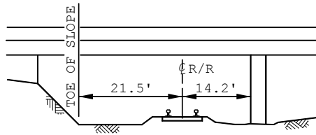
RAILROAD SINGLE TRACK
