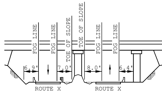
FREEWAY PIER MEDIAN WITH MOUNDED DIRT AROUND SUBSTRUCTURE
