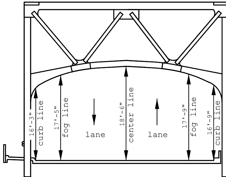
STEEL TRUSS
