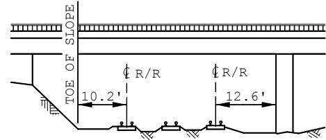
RAILROAD MULTIPLE TRACK
