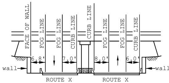
FREEWAY PIER MEDIAN WITH CONCRETE/DIRT FILL BETWEEN BARRIERS AROUND SUBSTRUCTURE
