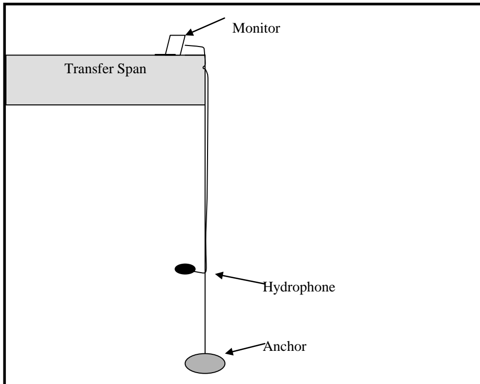
Figure 4: Diagram of hydrophone deployment configuration.
